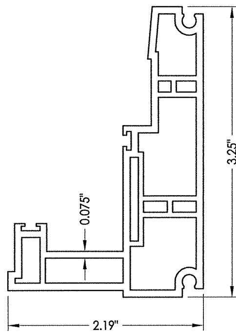
1 MAIN FRAME
