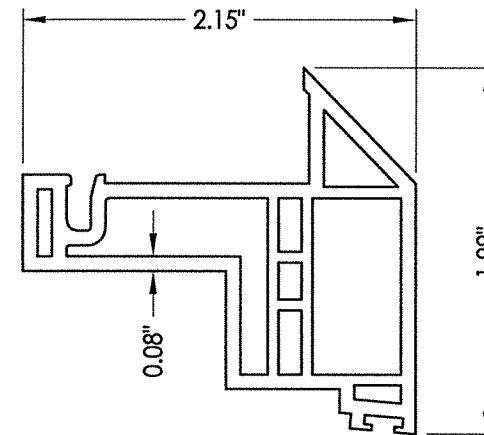
2 SASH FRAME
