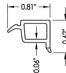
4 GLAZING BEAD
