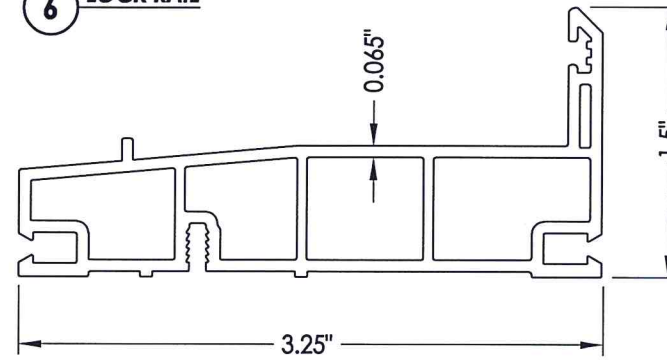
2 SILL
