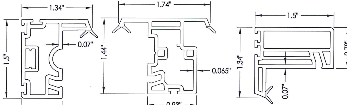
6 LOCK RAIL
