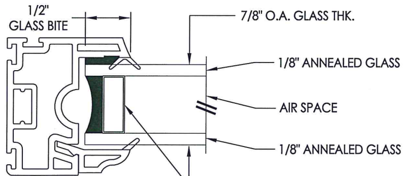
G1 GLAZING DETAIL - STAINLESS STEEL SPACER
