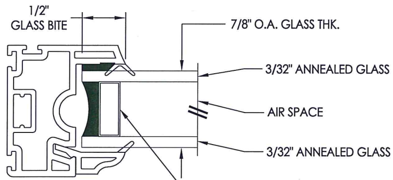
G1 GLAZING DETAIL - STAINLESS STEEL SPACER
