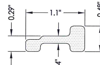
15 REINFORCEMENT Stile/ Rail
