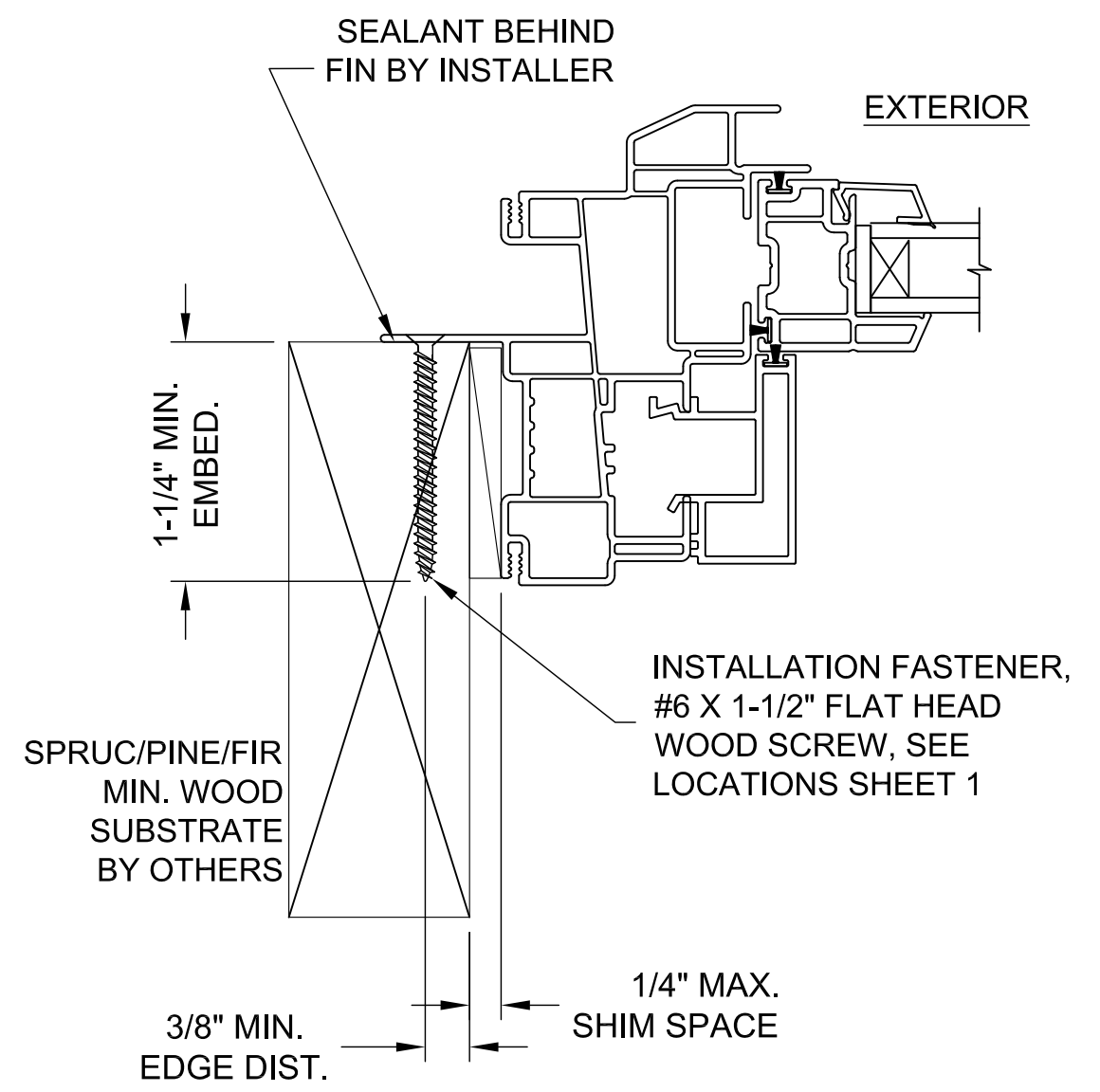
TYPICAL JAMB HORIZONTAL SECTION
