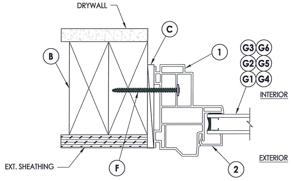
1 2 HORIZONTAL CROSS SECTION
