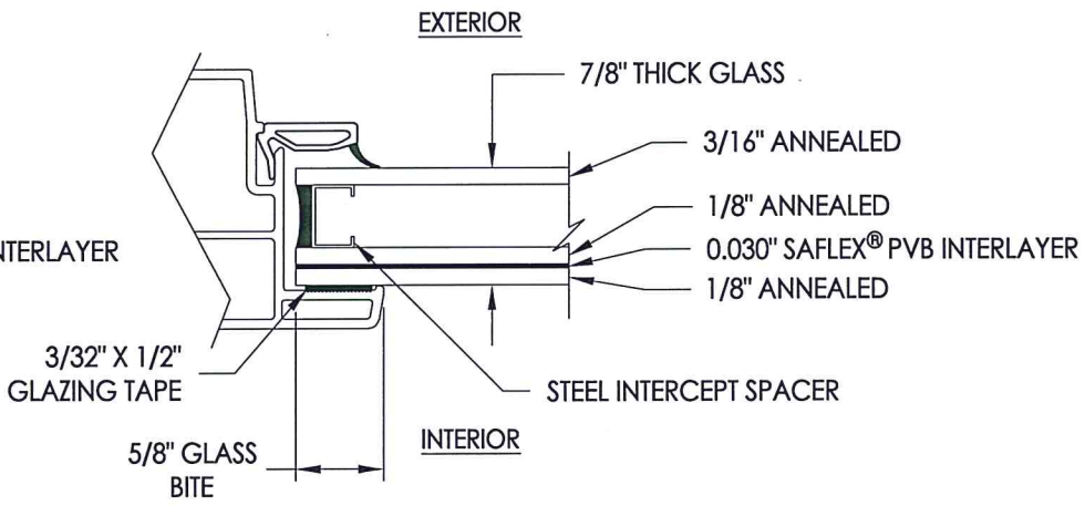
G6 GLAZING DETAIL
