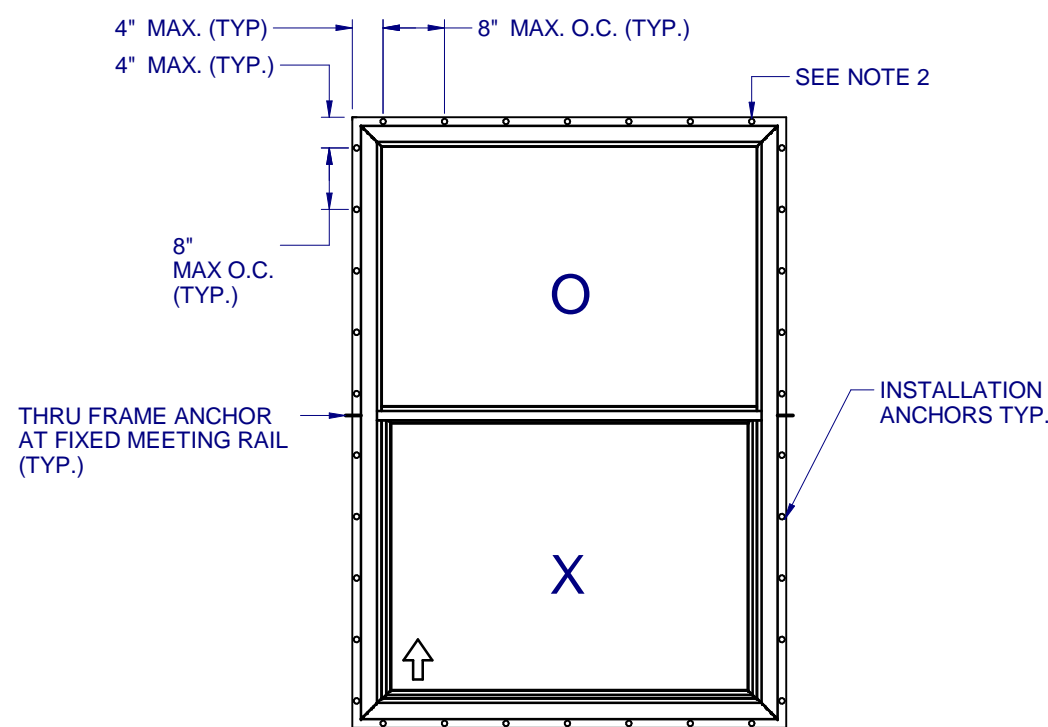
ANCHOR LAYOUT - (FIN)
