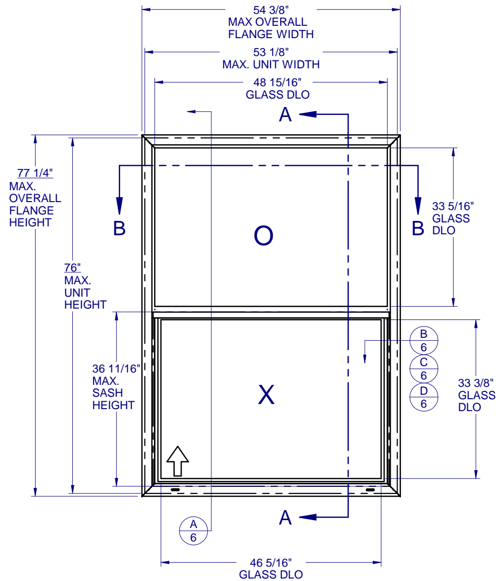
SYSTEM 1 (CAR 138-1007) MAXIMUM ALLOWABLE DESIGN PRESSURE: +50/-50 PSF
