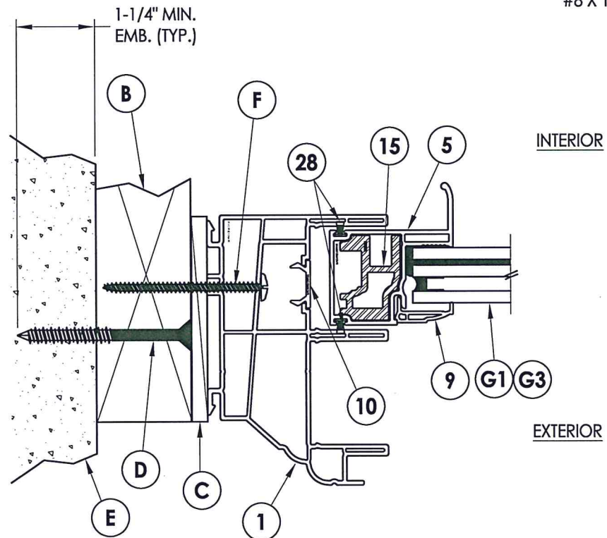
1 HORIZONTAL CROSS SECTION 2X Buck Construction
