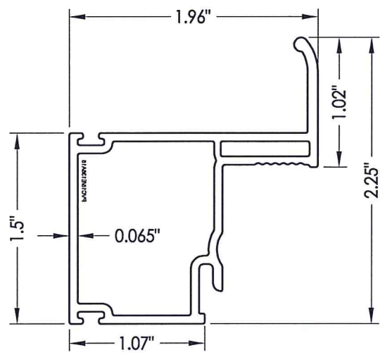
5 HANDLE SASH
