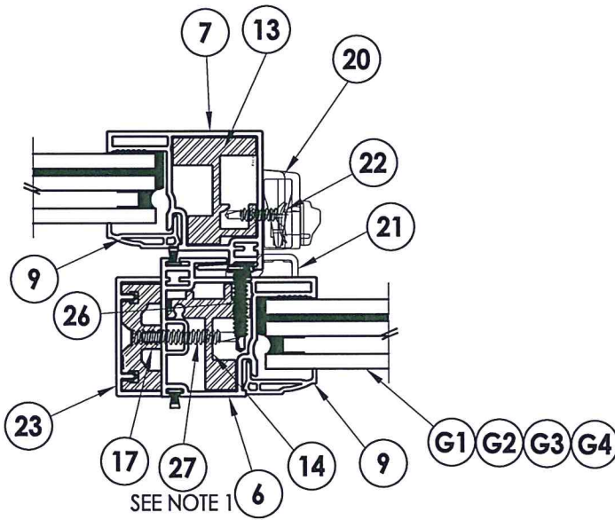
1 HORIZONTAL CROSS SECTION 2X Buck Construction
