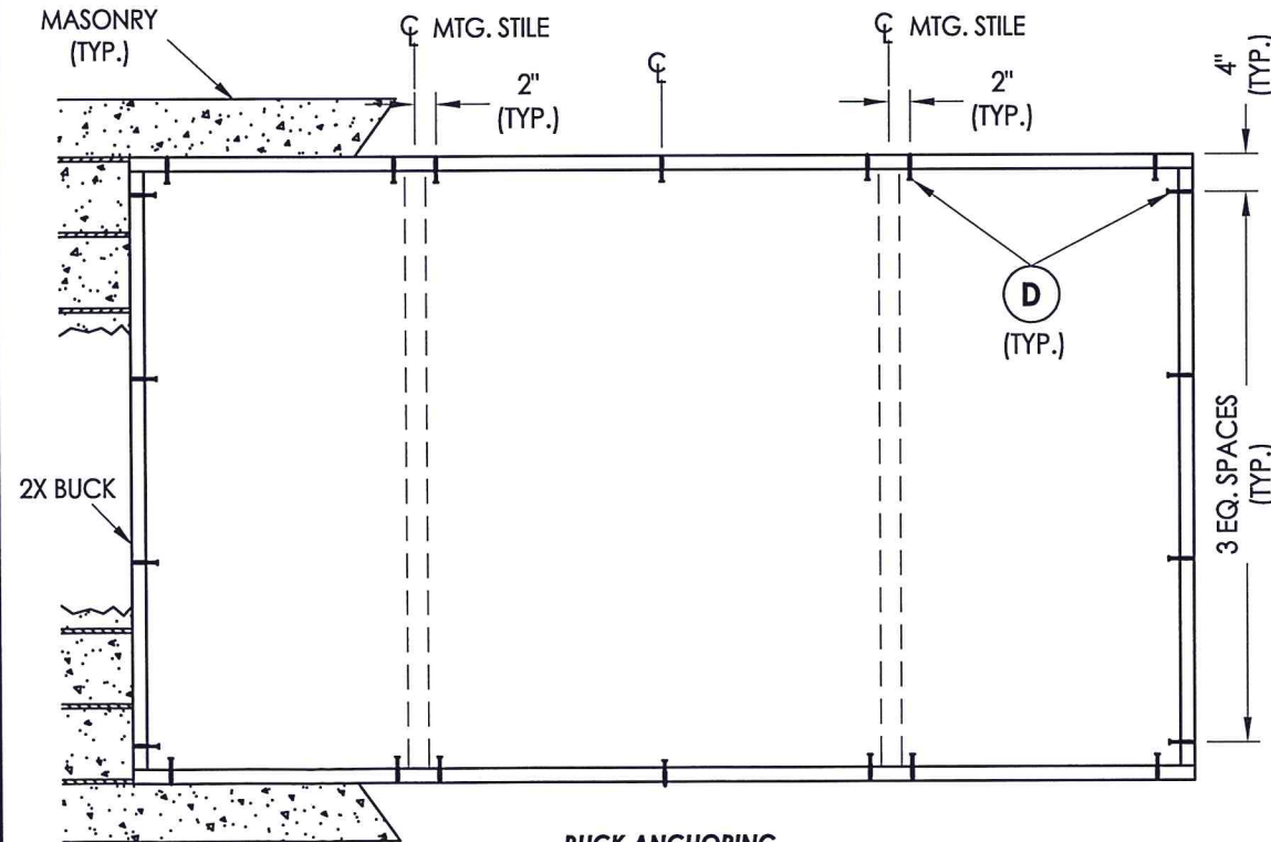
BUCK ANCHORING 1/4-1/2-1/4
