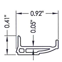
9 GLAZING BEAD
