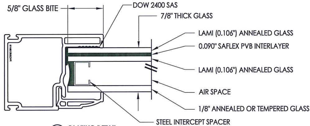
G3 GLAZING DETAIL
