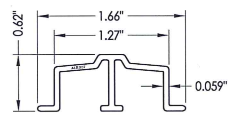
12 SILL ROLLER TRACK
