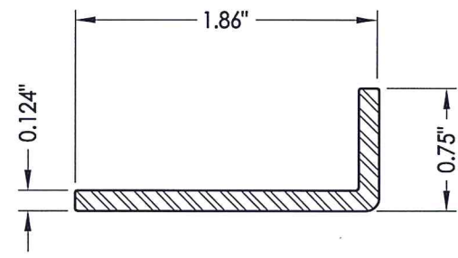
16 REINFORCEMENT
