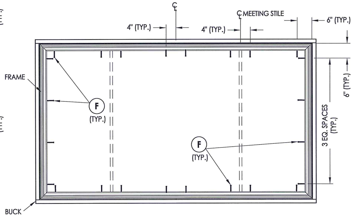
FRAME ANCHORING 1/4-1/2-1/4
