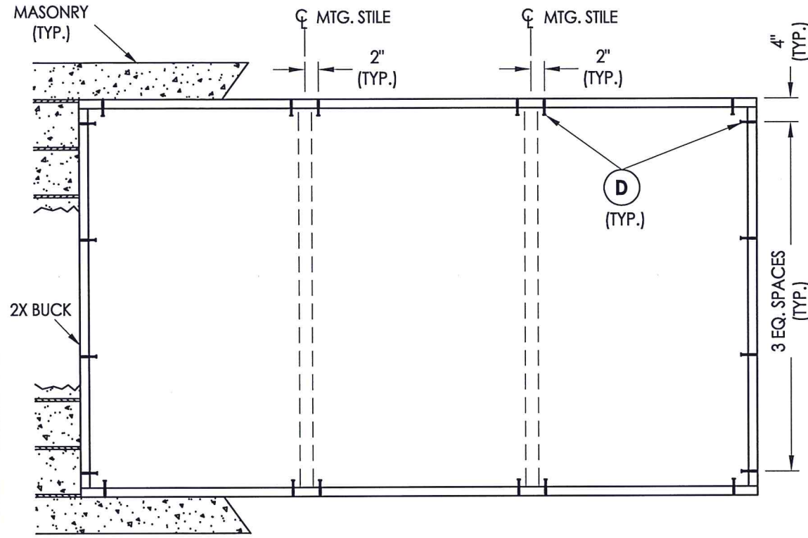
BUCK ANCHORING 1/3-1/3-1/3
