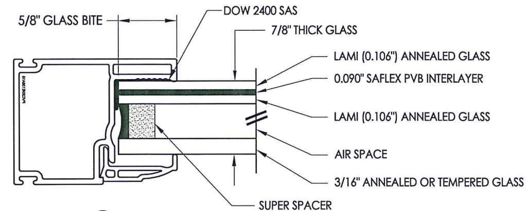
G4 GLAZING DETAIL
