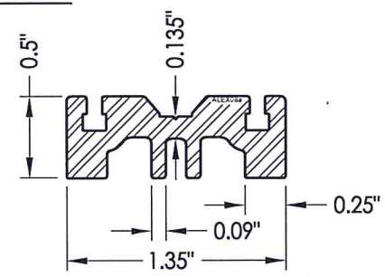
17 REINFORCEMENT
