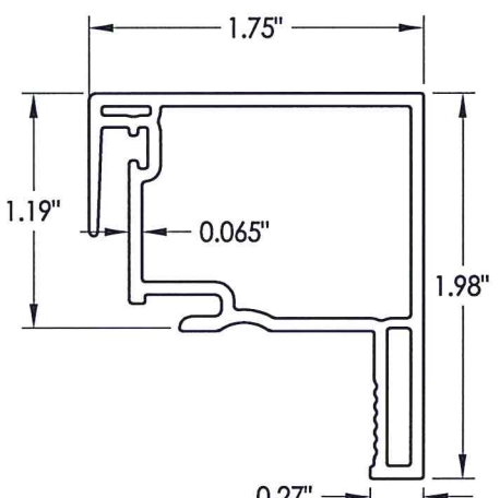
7 LOCK RAIL
