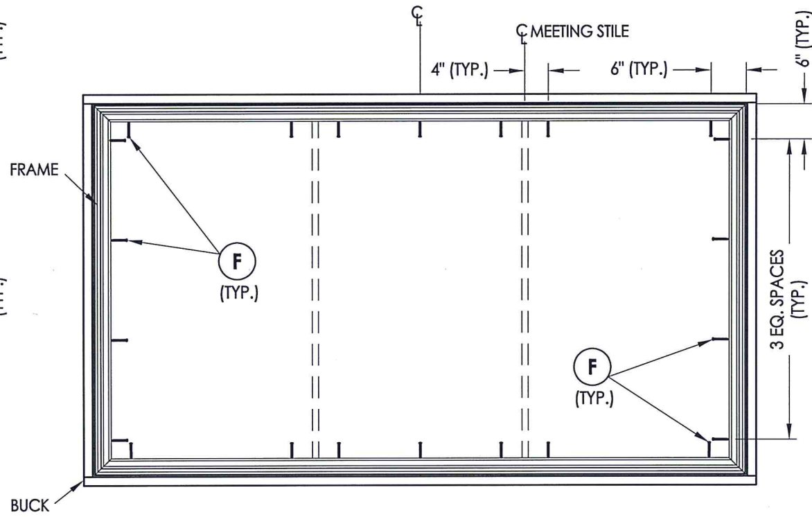
FRAME ANCHORING 1/3-1/3-1/3
