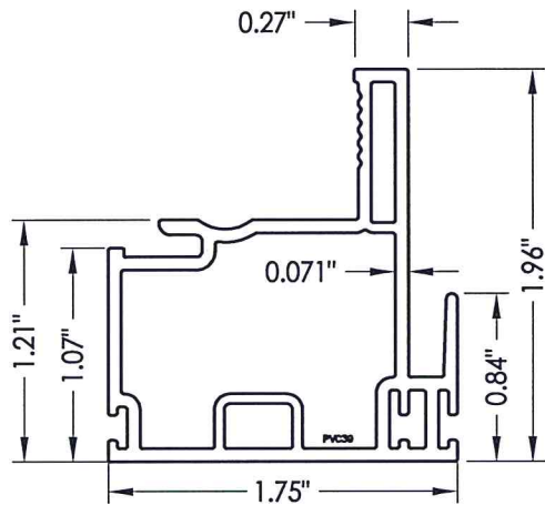
6 KEEPER RAIL
