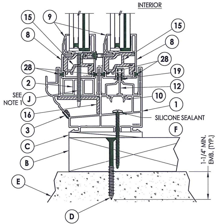
2 VERTICAL CROSS SECTION 3 2X Buck Construction
