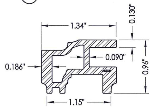
15 REINFORCEMENT
