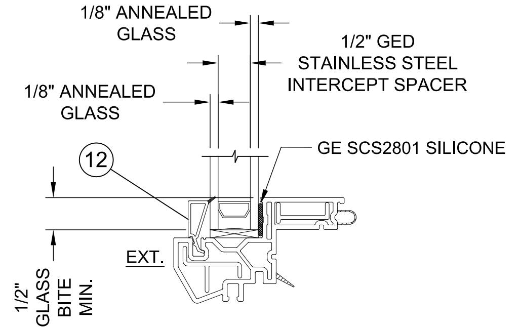
TYPICAL MIN. GLAZING DETAIL
