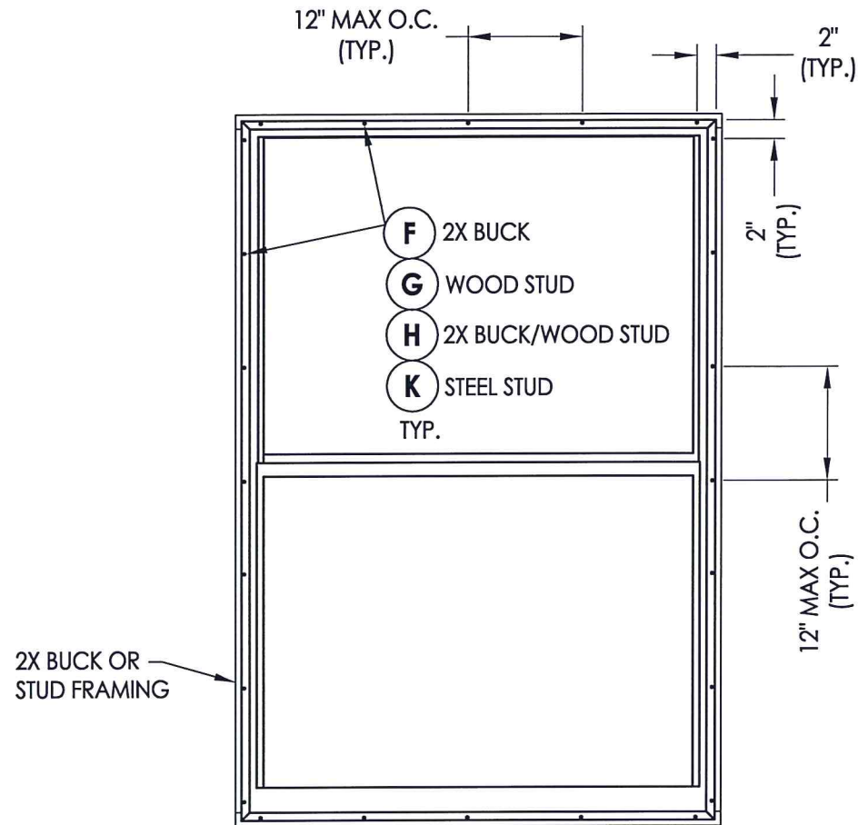
FRAME ANCHORING
