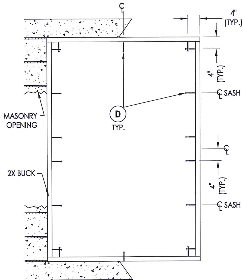
BUCK ANCHORING
