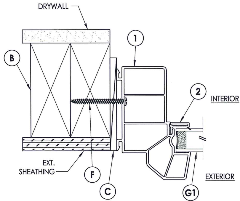
1 HORIZONTAL CROSS SECTION 2
