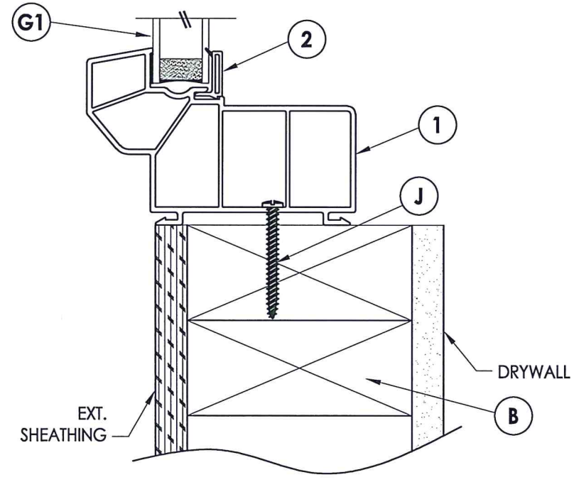
2 VERTICAL CROSS SECTION
