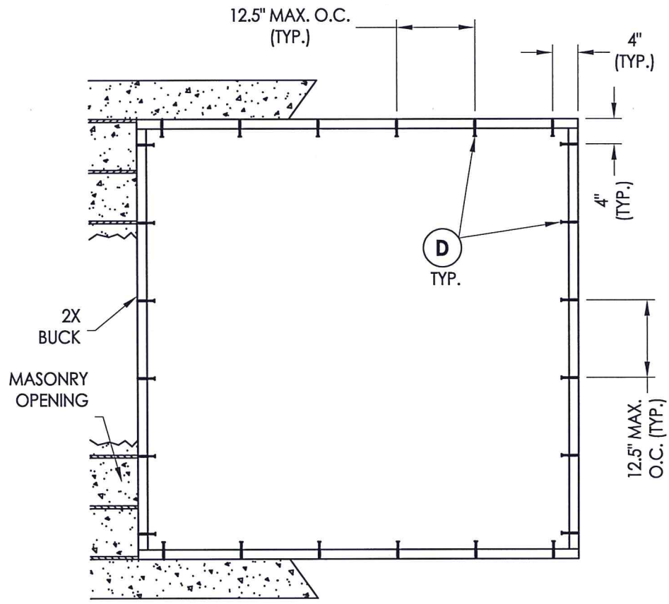
BUCK ANCHORING 2X BUCK MASONRY CONSTRUCTION
