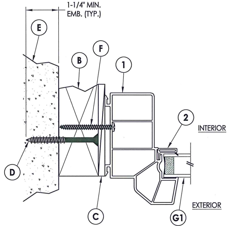
3 HORIZONTAL CROSS SECTION 2 Shown w/ 2X Buck Masonry Construction
