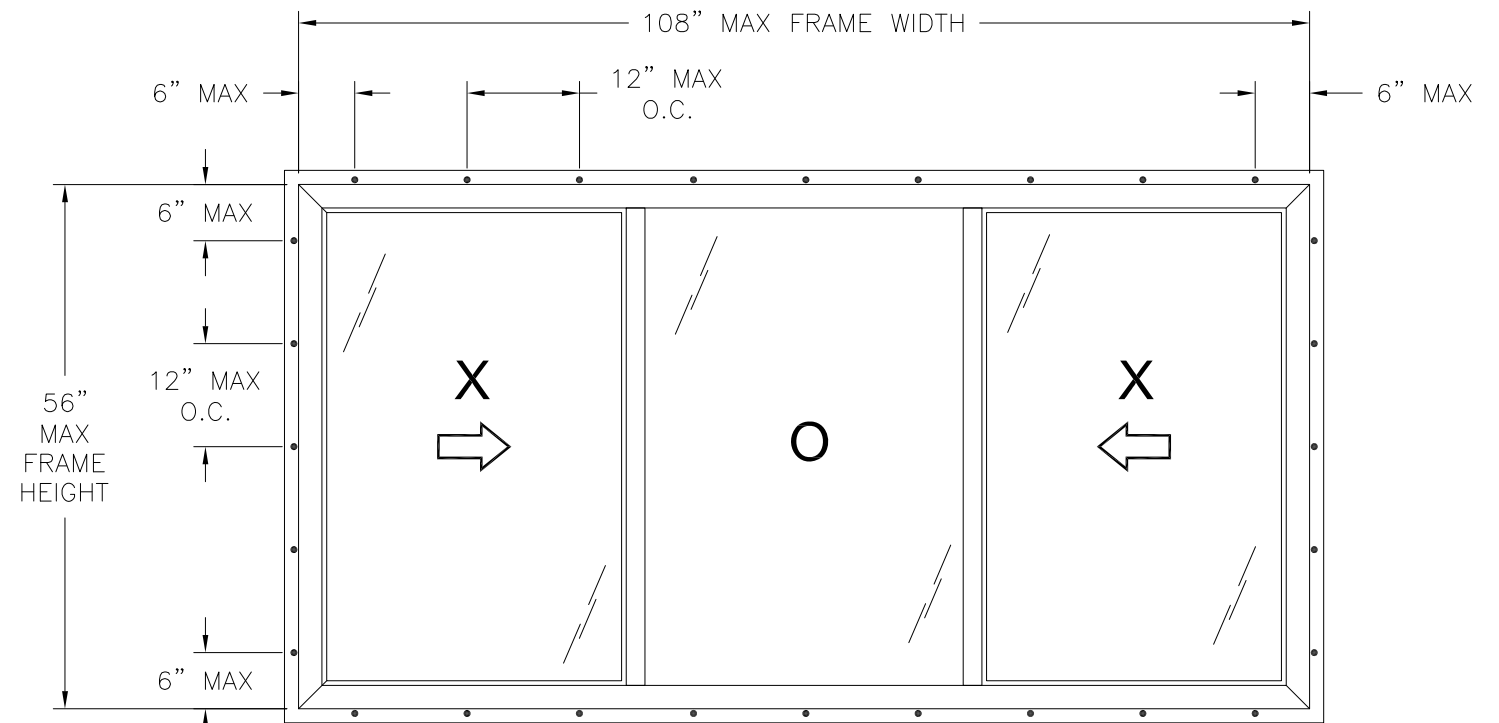
SERIES ENDURA 120/130 HORIZONTAL SLIDING WINDOW EXTERIOR VIEW FIN INSTALLATION
