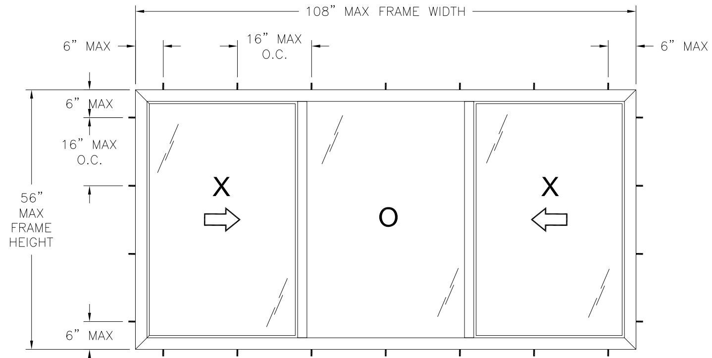
SERIES ENDURA 120/130 HORIZONTAL SLIDING WINDOW EXTERIOR VIEW FRAME INSTALLATION
