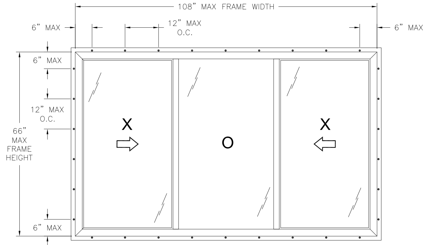
SERIES ENDURA 120/130 HORIZONTAL SLIDING WINDOW EXTERIOR VIEW FIN INSTALLATION
