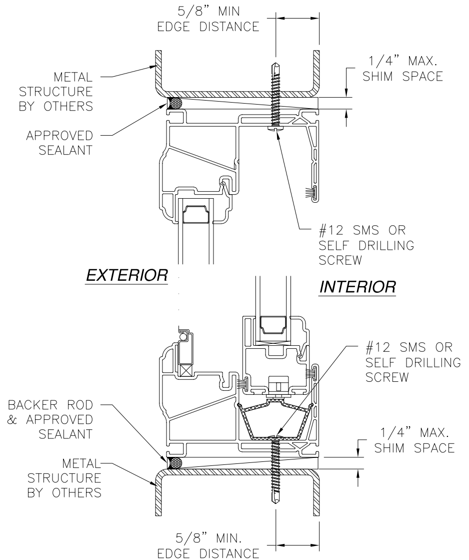
VERTICAL CROSS SECTION METAL STRUCTURE INSTALLATION
