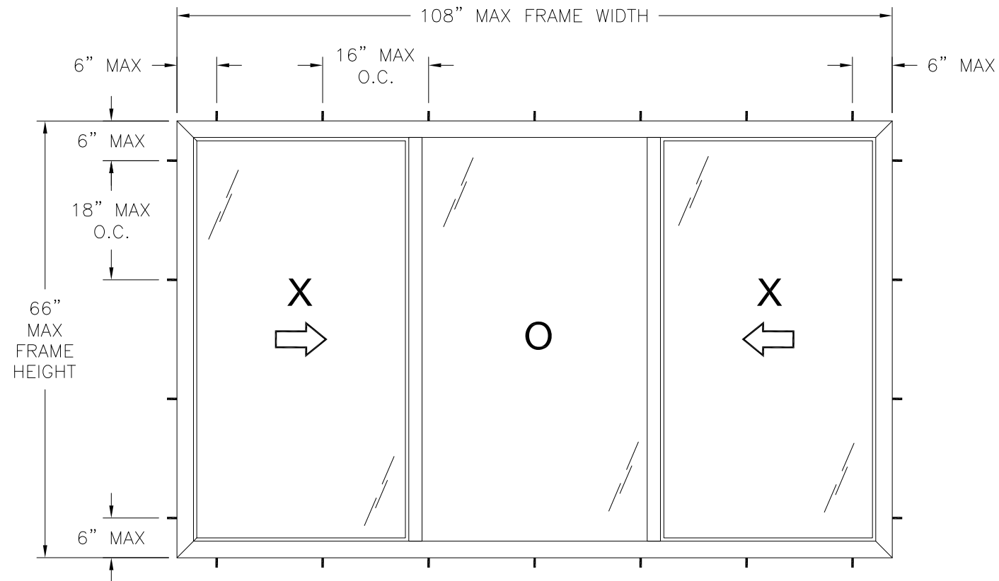
SERIES ENDURA 120/130 HORIZONTAL SLIDING WINDOW EXTERIOR VIEW FRAME INSTALLATION
