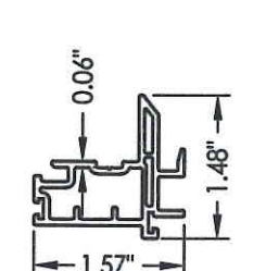
4 MEETING RAIL
