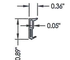
12 GLAZING BEAD
