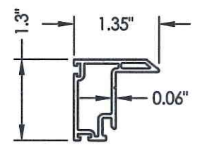
5 SASH STILE Small
