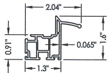
8A BOTTOM LIFT RAIL Medium
