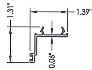
7 HEAD INSERT
