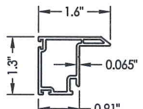
5A SASH STILE Medium
