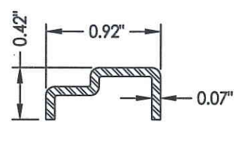
14 REINFORCEMENT Meeting Rail
