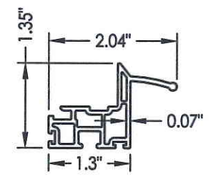
8 BOTTOM LIFT RAIL Small
