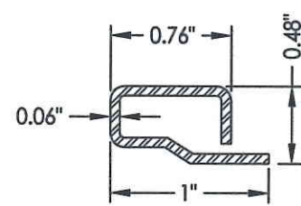
16 REINFORCEMENT SM Stiles
