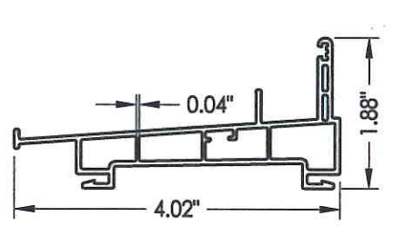
2 SILL
