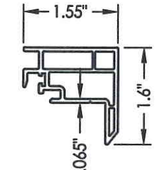
3A LOCK RAIL Medium
