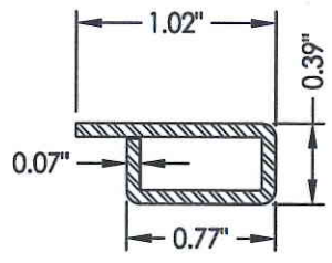
15 REINFORCEMENT Lock Rail
