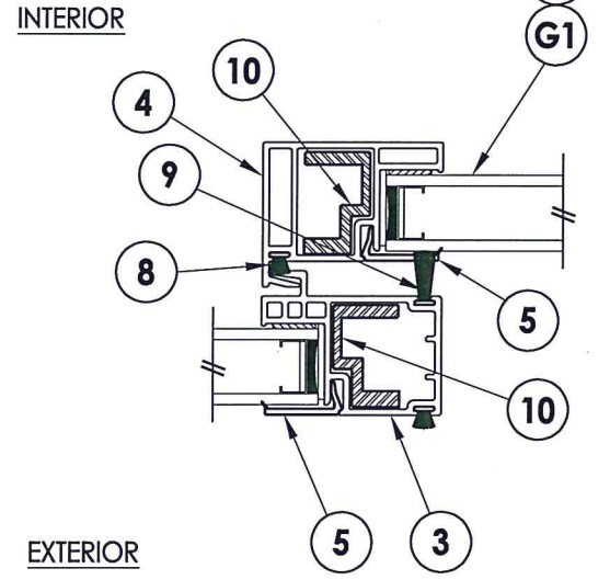
2 2 HORIZONTAL CROSS SECTION
