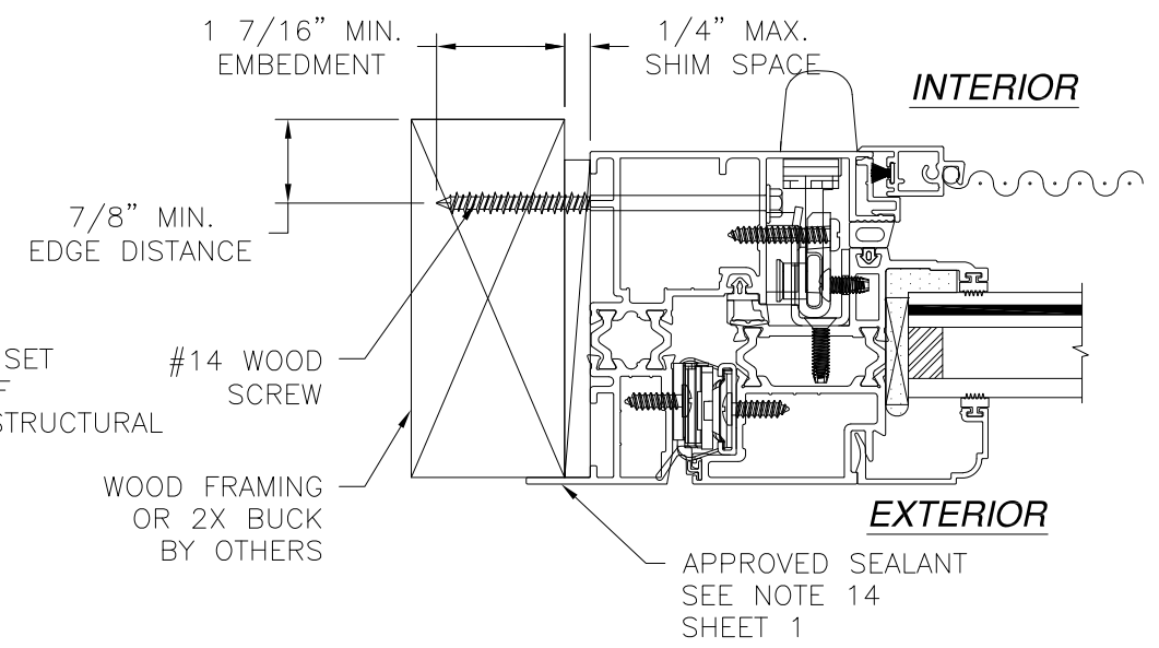
B/7 JAMB INSTALLATION DETAIL WOOD FRAMING OR 2X BUCK INSTALLATION
