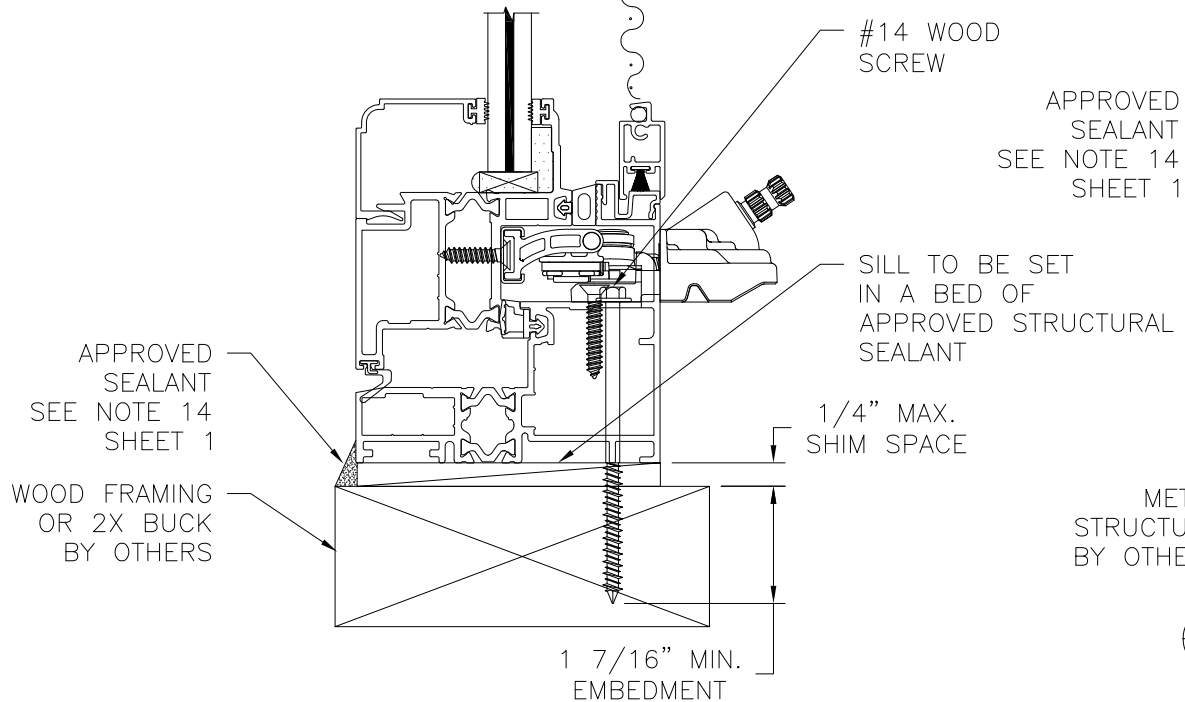
A/5 VERTICAL CROSS SECTION WOOD FRAMING OR 2X BUCK INSTALLATION
