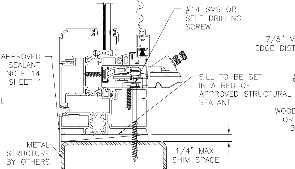
A/7 VERTICAL CROSS SECTION METAL STRUCTURE INSTALLATION
