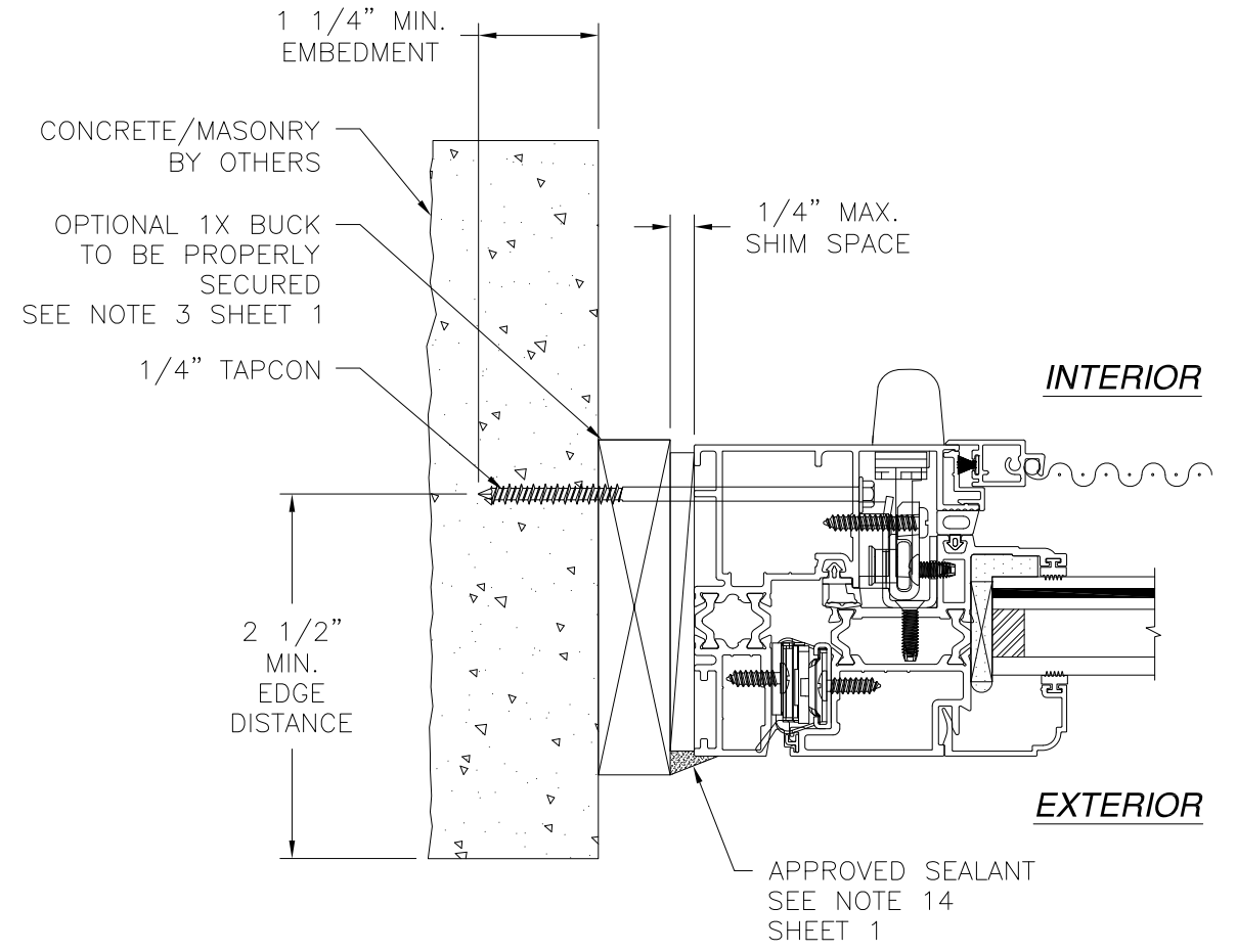
B 6 JAMB INSTALLATION DETAIL CONCRETE/MASONRY INSTALLATION
