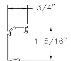
②⑩ GLASS STOP ALUMINUM 6063-T6 .050" THICK
