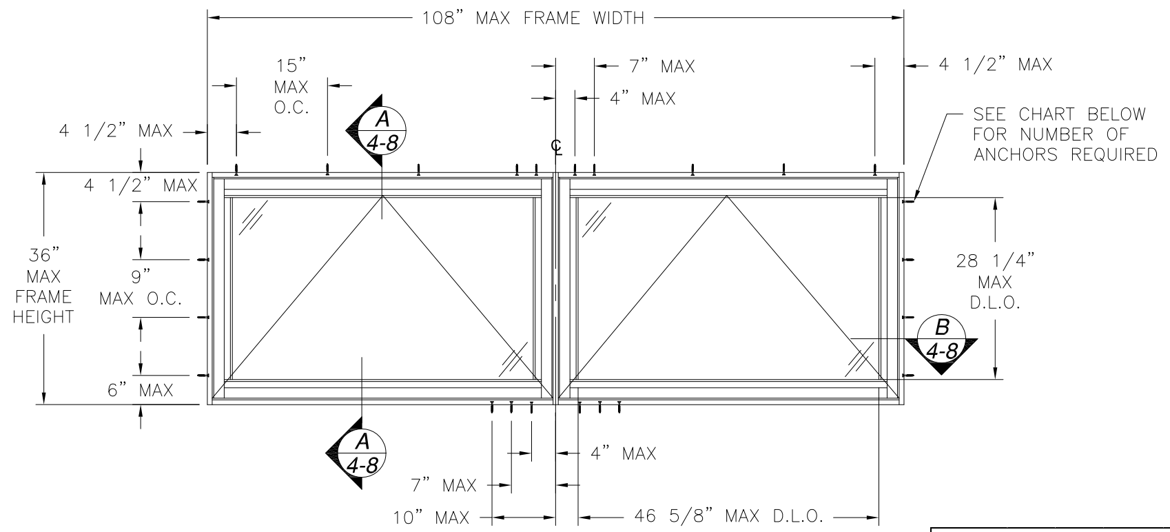
SERIES 9066 AWNING TWIN WINDOW EXTERIOR VIEW
