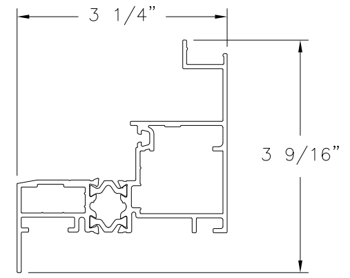
② FLANGE FRAME ALUMINUM 6063-T6 .065" THICK
