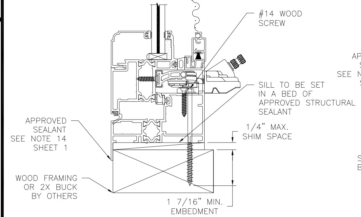
A/7 VERTICAL CROSS SECTION WOOD FRAMING OR 2X BUCK INSTALLATION
