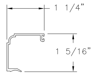
①⑨ GLASS STOP ALUMINUM 6063-T6 .050" THICK
