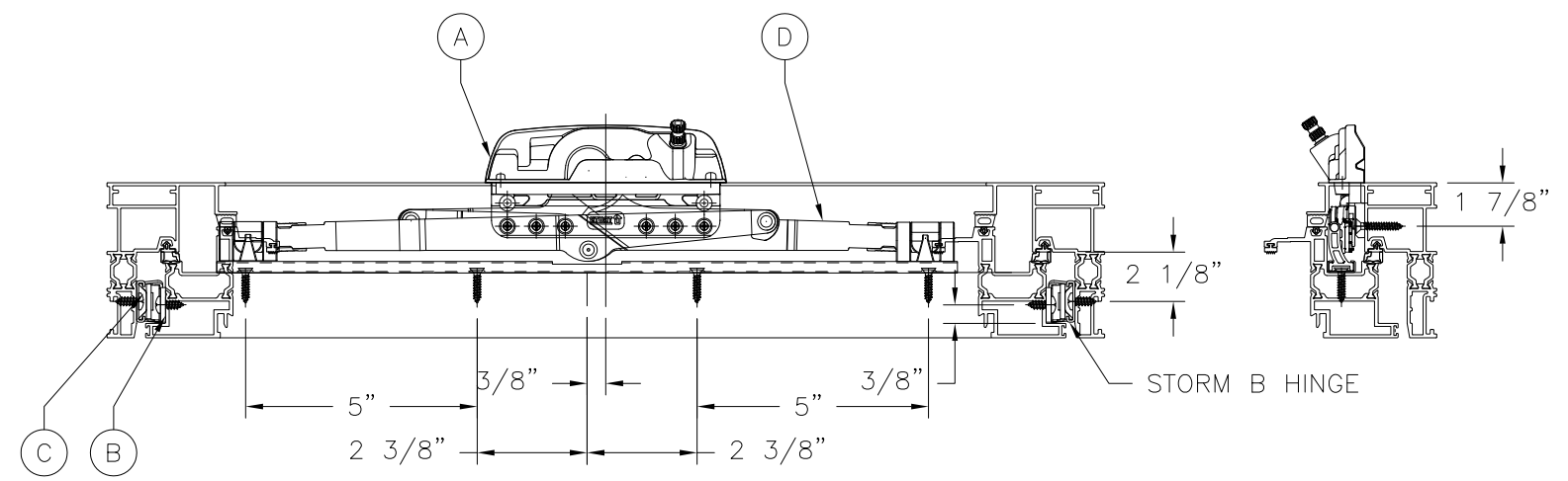
HARDWARE DETAIL
