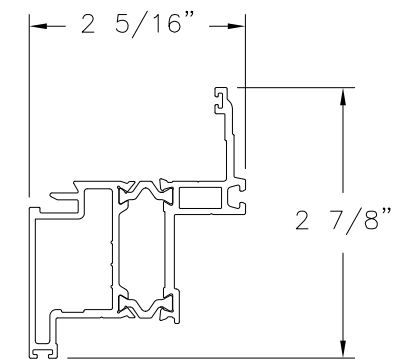
③ SASH ASSEMBLY ALUMINUM 6063-T6 .070" THICK
