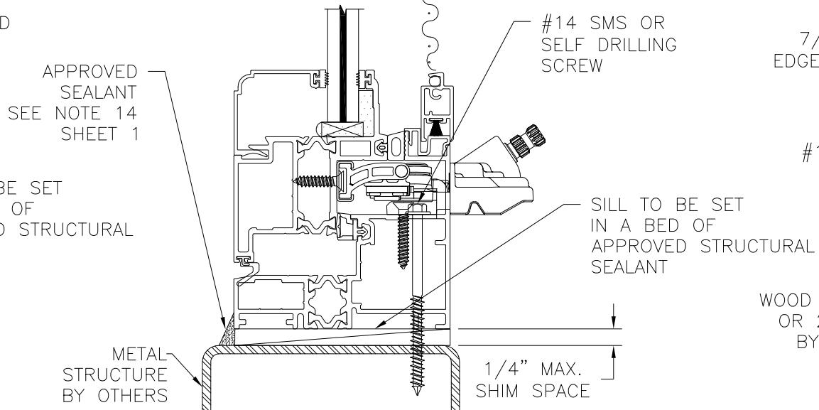
A/5 VERTICAL CROSS SECTION METAL STRUCTURE INSTALLATION
