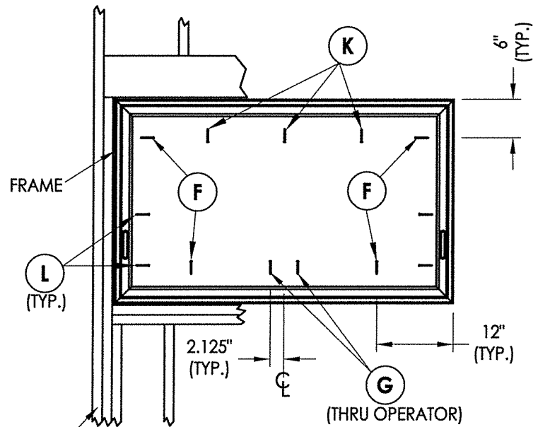
SNUBBER LOCATIONS 3 Req'd
