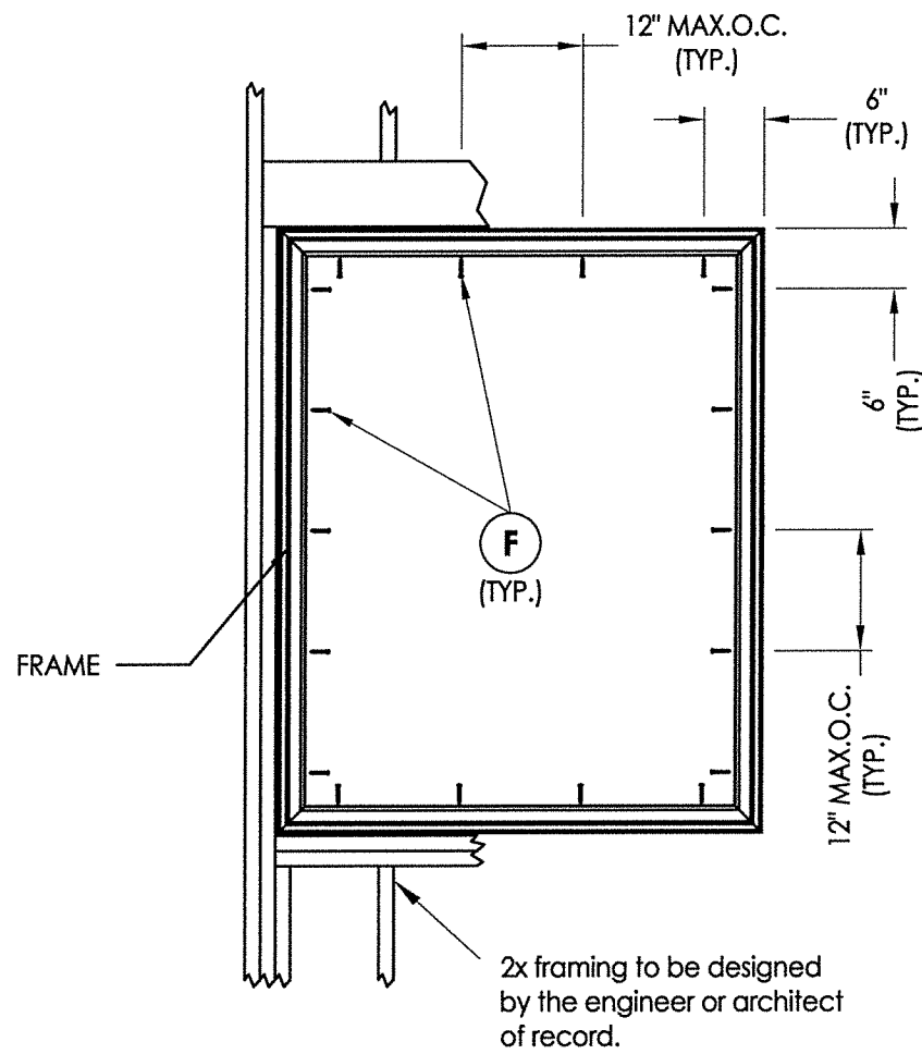
FRAME ANCHORING 48" X 60" MAX
