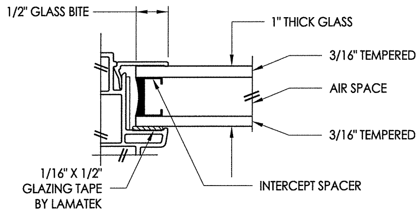
G4 GLAZING DETAIL
