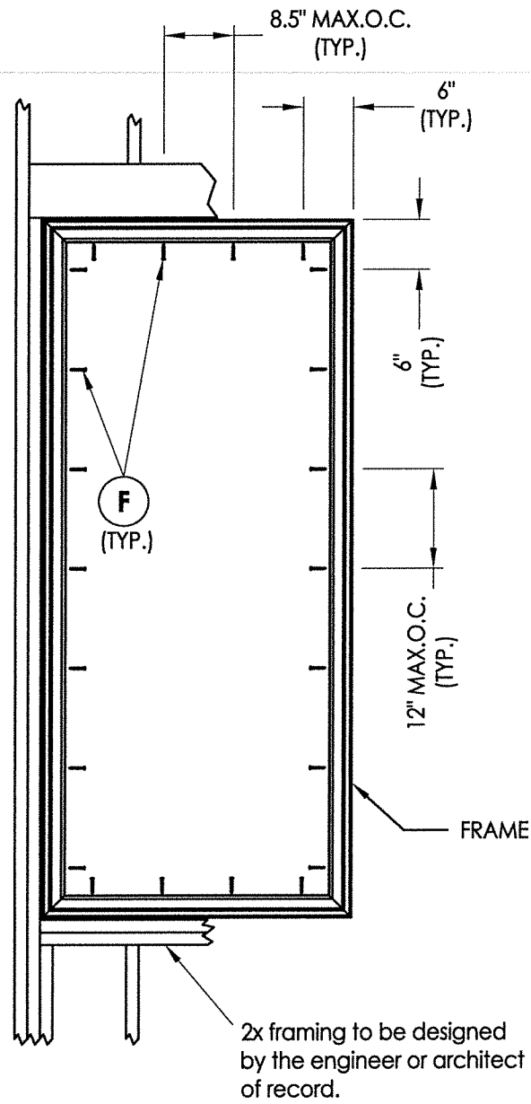
FRAME ANCHORING 37" X 84" MAX
