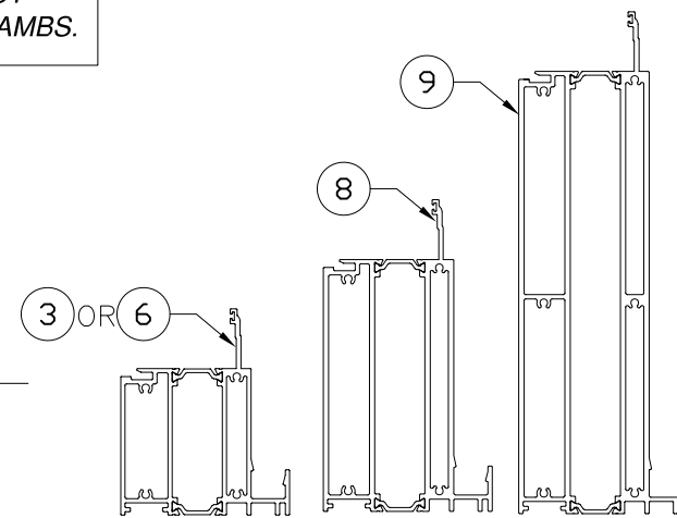
OTHER HEIGHTS RAILS MAY BE USED IN ONE OR ALL FRAME LOCATIONS. SHOWN HALF SCALE.
