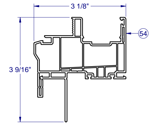
PVC FRAME FIN/FLANGE H-6231
