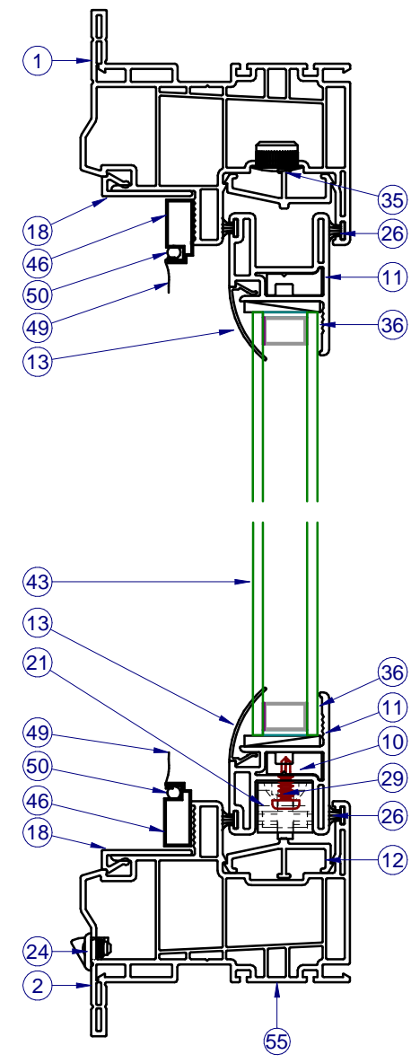
SECTION VIEW D-D
