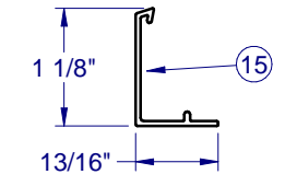
PVC MTG RAIL COVER S-6228
