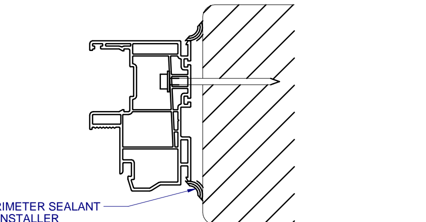
D HORIZONTAL SECTION 8 BOX FRAME INSTALLATION HEAD AND SILL SIMILAR FOR BOX INSTALLATION
