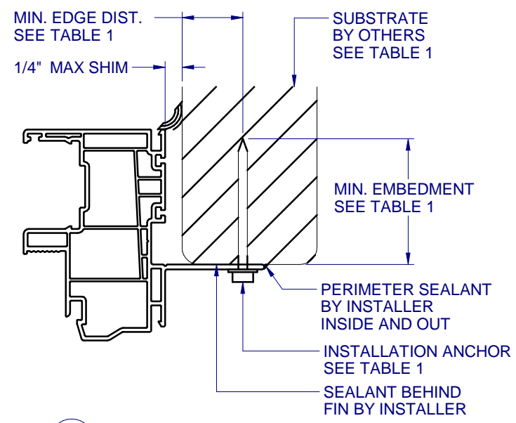
E HORIZONTAL SECTION 8 TYPICAL FIN ANCHORAGE HEAD AND SILL SIMILAR FOR FIN INSTALLATION
