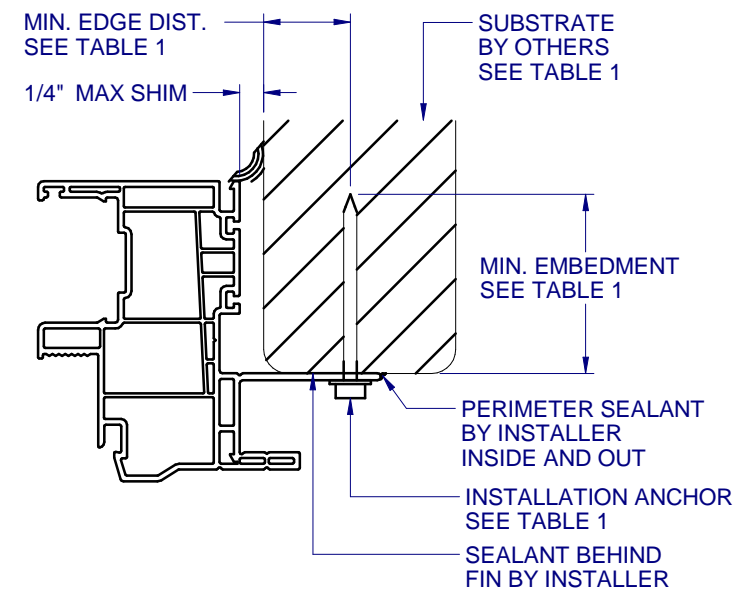
C HORIZONTAL SECTION 8 TYPICAL FIN ANCHORAGE HEAD AND SILL SIMILAR FOR FIN INSTALLATION
