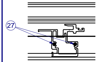
FIXED MEETING RAIL SCREWED TOGETHER WITH OUTERFRAME 1:8
