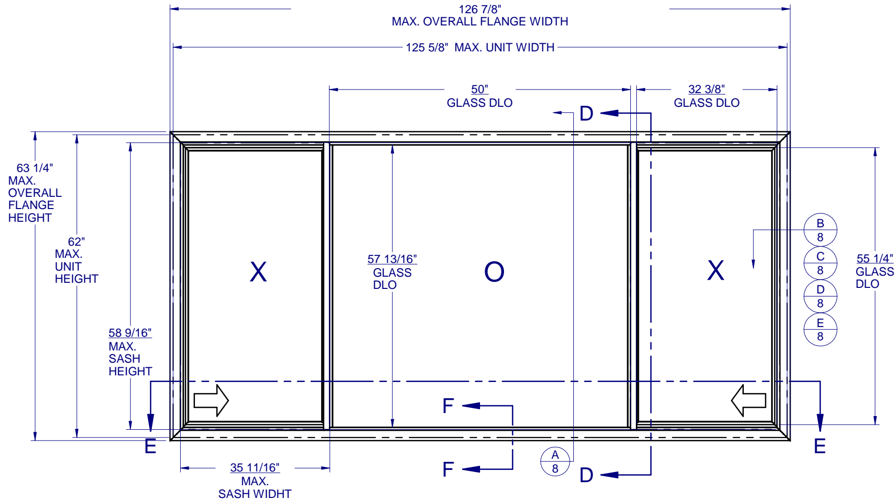
SYSTEM 2 (CAR 138-1018) MAXIMUM ALLOWABLE DESIGN PRESSURE: +30/-30 PSF
