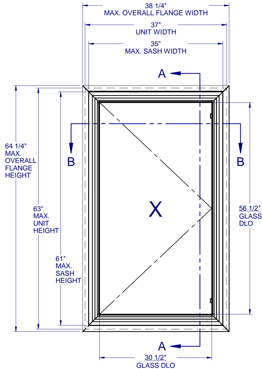
RIGHT HINGED - SHOWN ELEVATION B (CAR 138-275/138-731) MAXIMUM ALLOWABLE DESIGN PRESSURE: +65/-65 PSF
