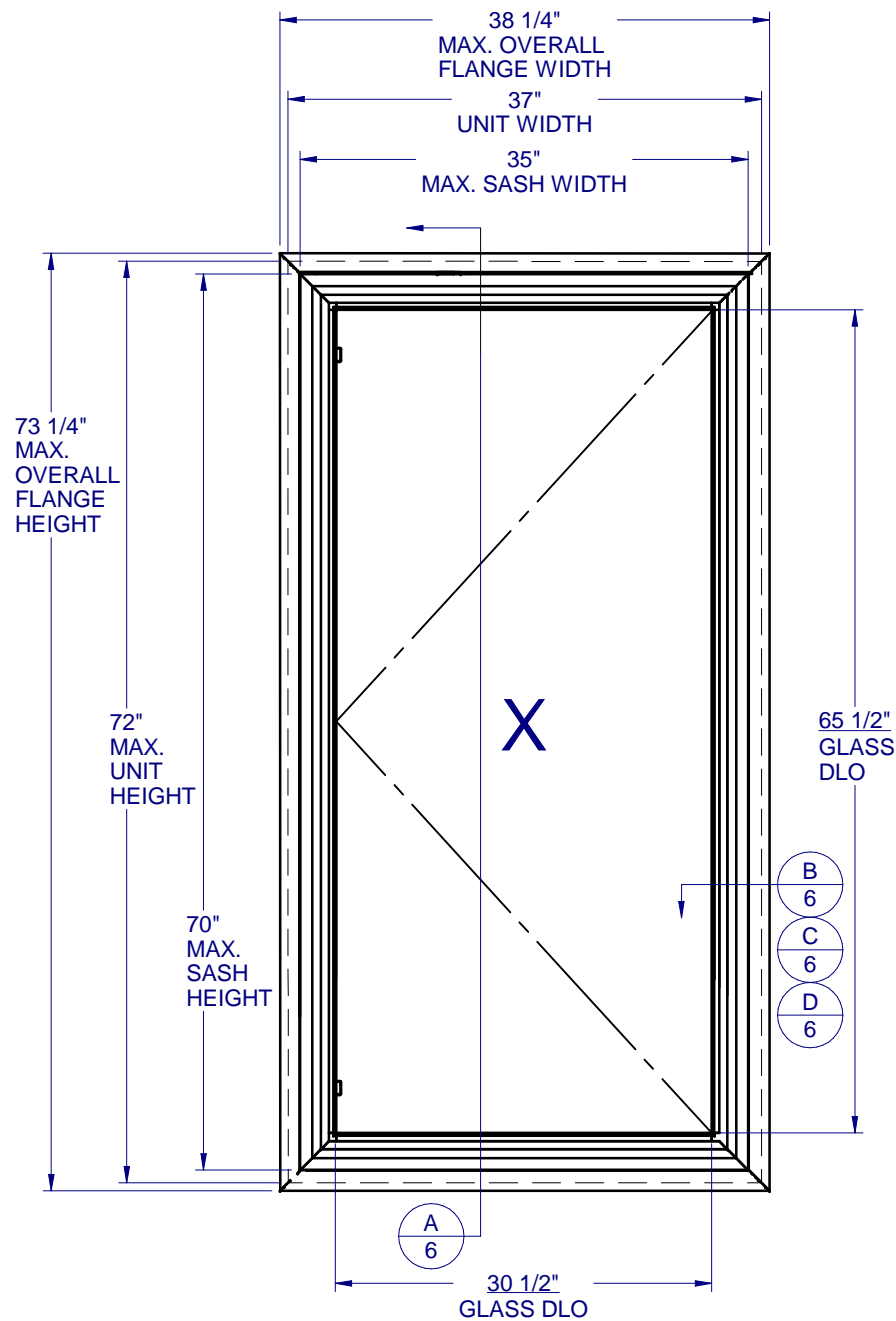
LEFT HINGED - SHOWN ELEVATION A (CAR 138-276/138-732)
