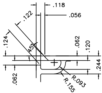
A Glazing Pocket 2 : 1
