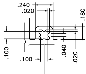
C Typ. Screw Boss 2 : 1
