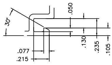
B Accessory Groove 2 : 1
