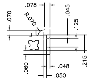
B Typ. Weather Stripping Pocket 2 : 1
