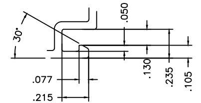
B Accessory Groove 2 : 1
