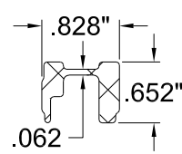
11 STILE REINFORCEMENT
