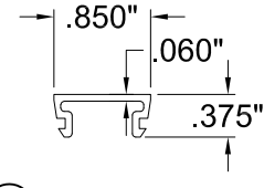
14 TOP PULL RAIL REINFORCEMENT
