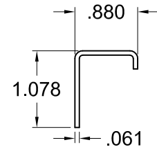
37 TILT LATCH REINFORCEMENT CLIP
