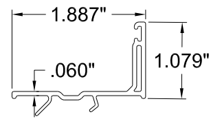
2 SILL ADAPTER
