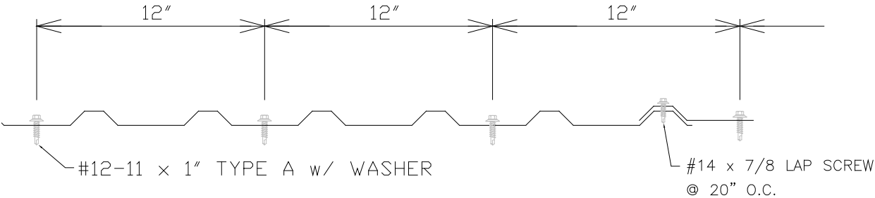
12"-12"-12" SCREW PATTERN
