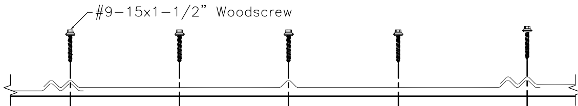
FASTENING PATTERN FOR 5V-CRIMP AT EAVE OR ENDLAP
