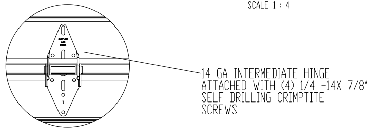
DETAIL J SCALE 1:4
