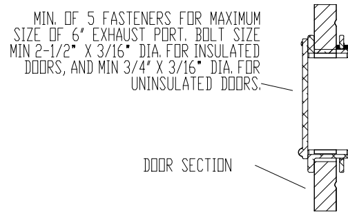
EXHAUST PORT DETAIL
