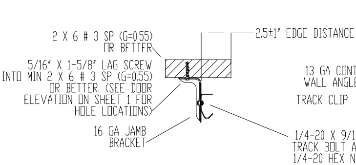
MOUNTING TO WOOD JAMB DETAIL
