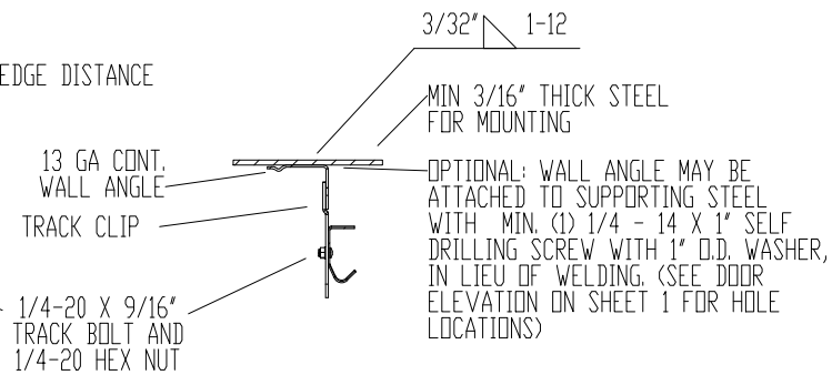
MOUNTING TO STEEL JAMB DETAIL
