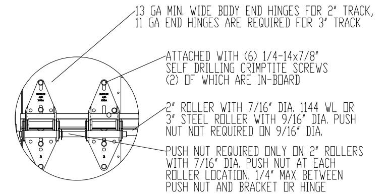
DETAIL I SCALE 1:4
