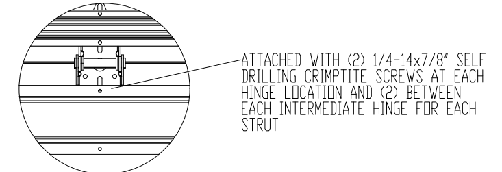
DETAIL L SCALE 1:4
