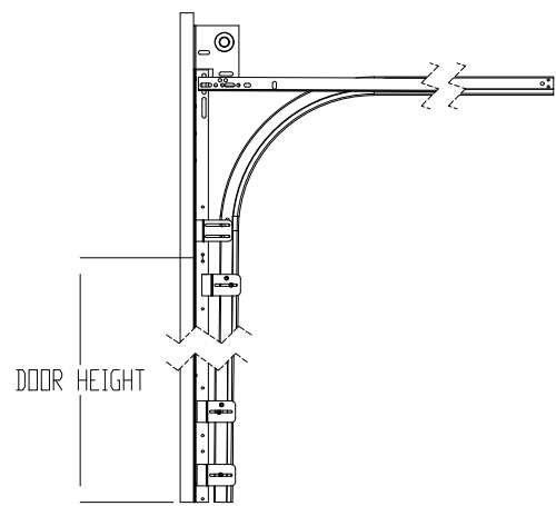
STANDARD LIFT TRACK DETAIL
