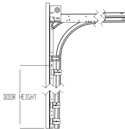
LOW HEADROOM TRACK DETAIL
