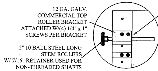
TYPICAL TOP FIXTURES N.T.S. ①
