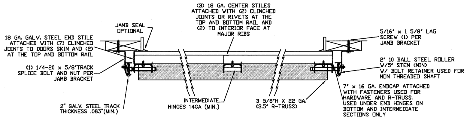
TRACK MOUNTING DETAIL N.T.S.
