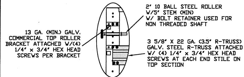
TYPICAL TOP FIXTURE N.T.S. 1
