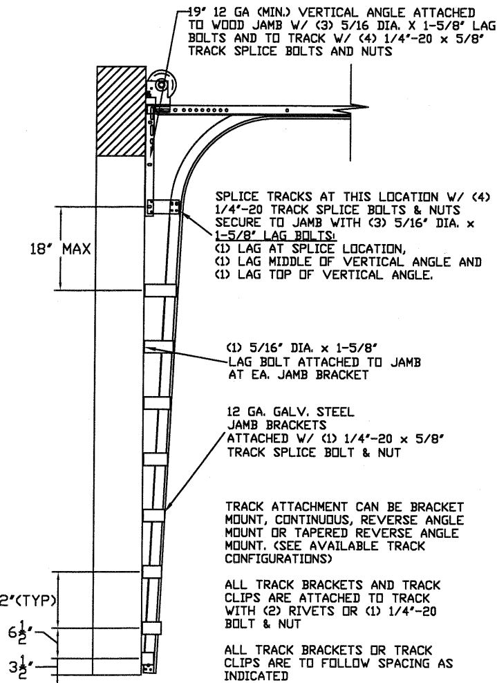
TRACK CONFIGURATION FOR UP TO 24' TALL DOORS
