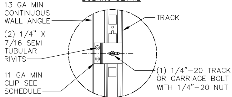
TYPICAL CLIP RIVETING DETAIL
