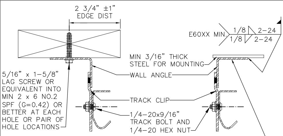
MOUNTING TO WOOD JAMB DETAIL
