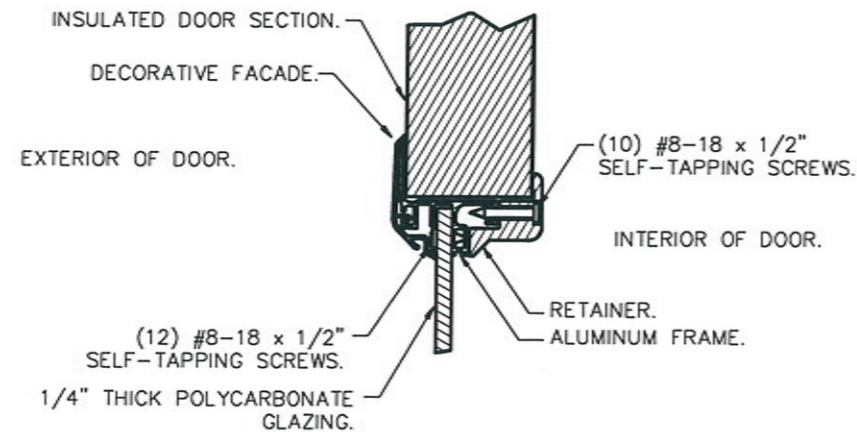
IMPACT-RESISTANT ASSEMBLY DETAILS DRAWING 104826-A
