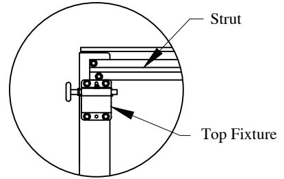
Strut above top fixture
