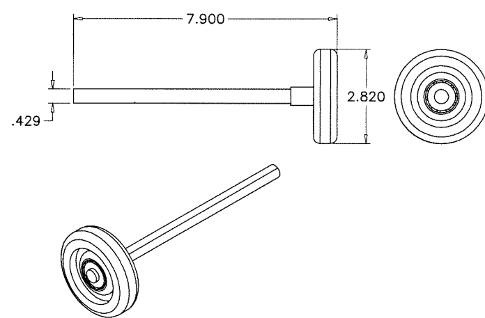
HURRICANE ROLLER-DF
