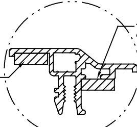
ALUMINUM FRAME (STATIC RATED ALTERNATE FRAME OPTION) DETAIL F
