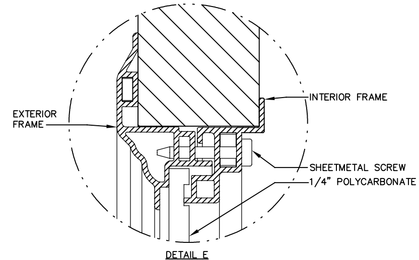
DETAIL E
