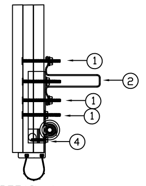
DETAIL A TYPICAL BOTTOM SECTION CONSTRUCTION
