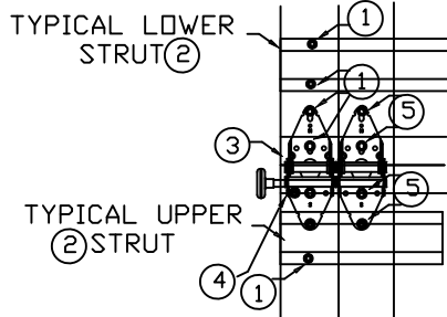
DETAIL G TYPICAL END STILE ATTACHMENT
