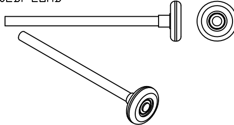
DETAIL Q 2" NYLON PRECISION BEARING HIGH STRENGTH ROLLER 9-1/2" ZINC PLATED HIGH STRENGTH STEM 100LB. LOAD
