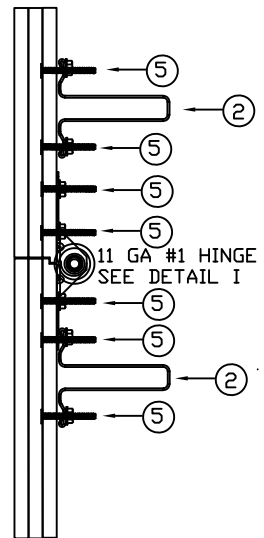
DETAIL B INTERIOR STILES TYPICAL SECTION CONSTRUCTION
