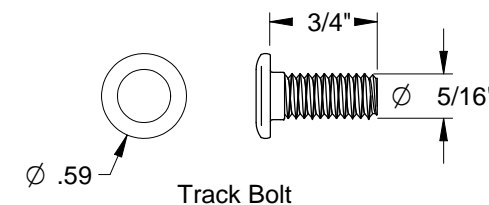
Track Bolt
