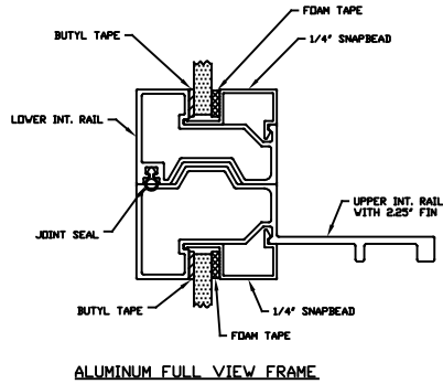
ALUMINUM FULL VIEW FRAME
