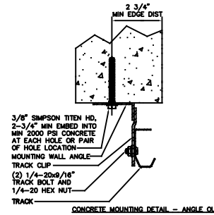
CONCRETE MOUNTING DETAIL - ANGLE CUT
