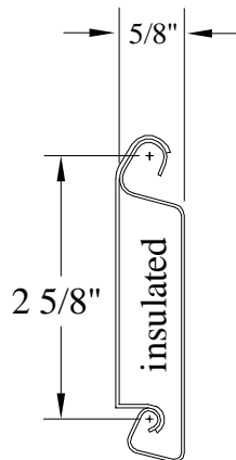
Steel Slat Thickness .024/.024 insulated
