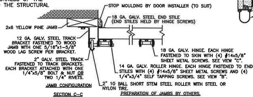
JAMB CONFIGURATION SECTION C-C
