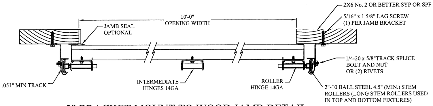
2" BRACKET MOUNT TO WOOD JAMB DETAIL N.T.S.
