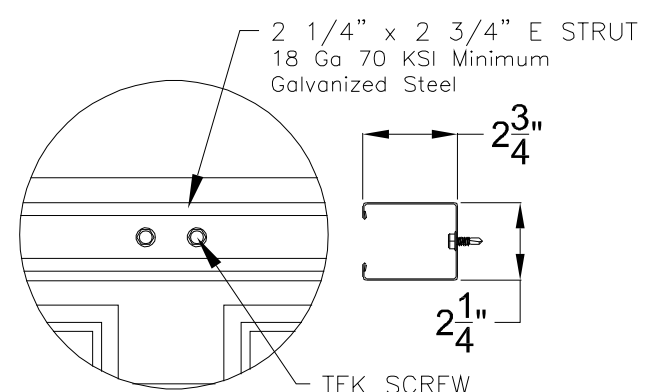
DETAIL J
