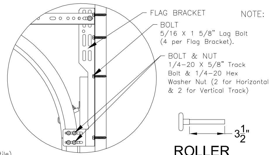
DETAIL H
