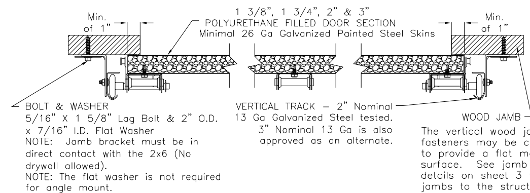
DETAIL H
