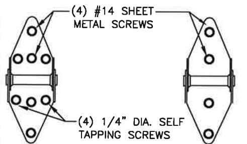
14 GA. END HINGE 14 GA. INTERMEDIATE HINGE
