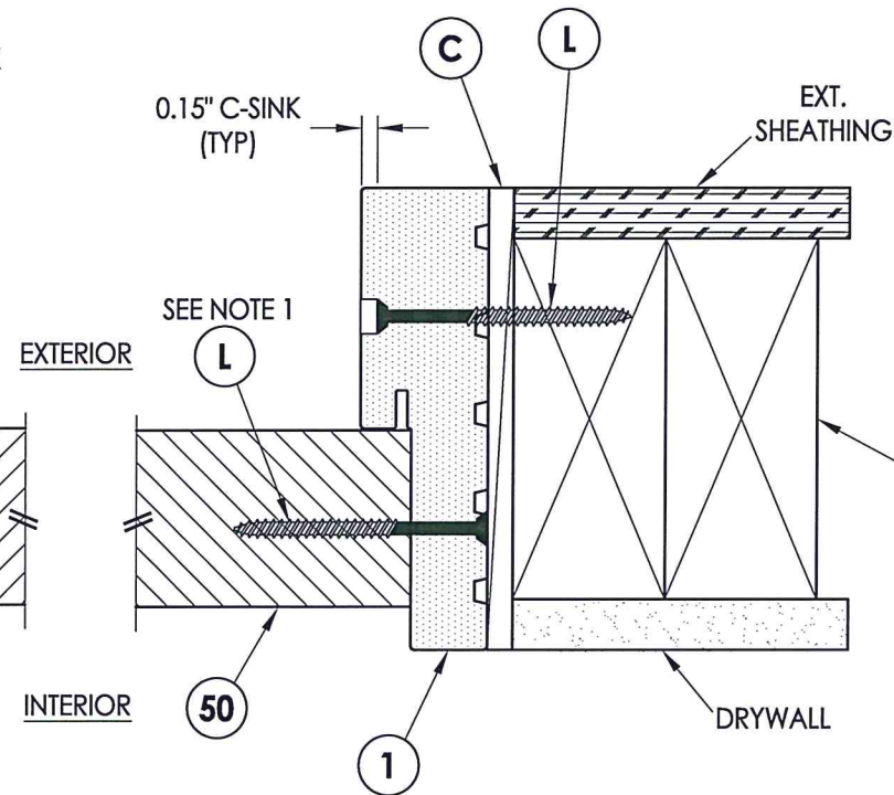
2 HORIZONTAL CROSS SECTION 5 Shown w/ 2X Buck Inswing shown (Outswing similar)
