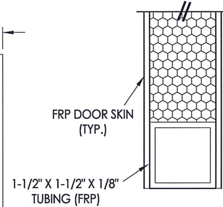
4 2 VERTICAL CROSS SECTION
