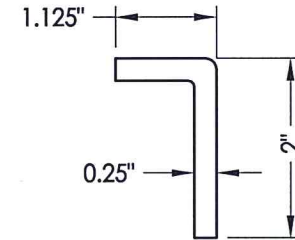
3 ASTRAGAL (FRP)
