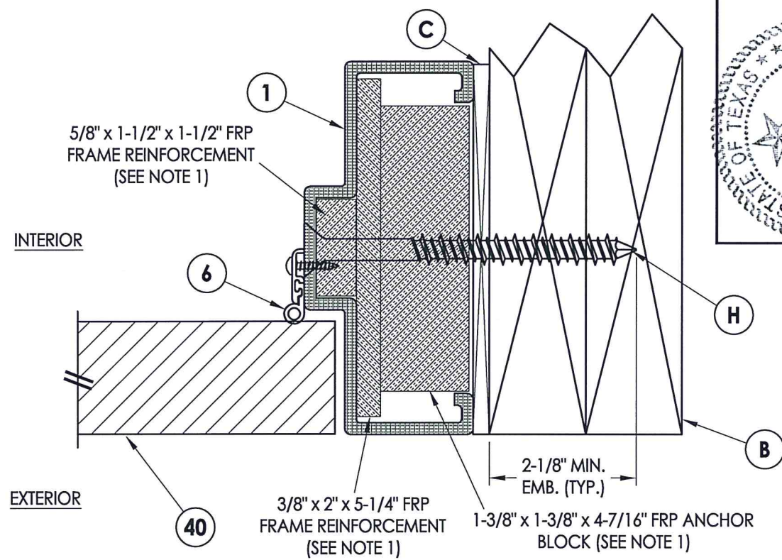
3 HORIZONTAL CROSS SECTION 3 Outswing configuration
