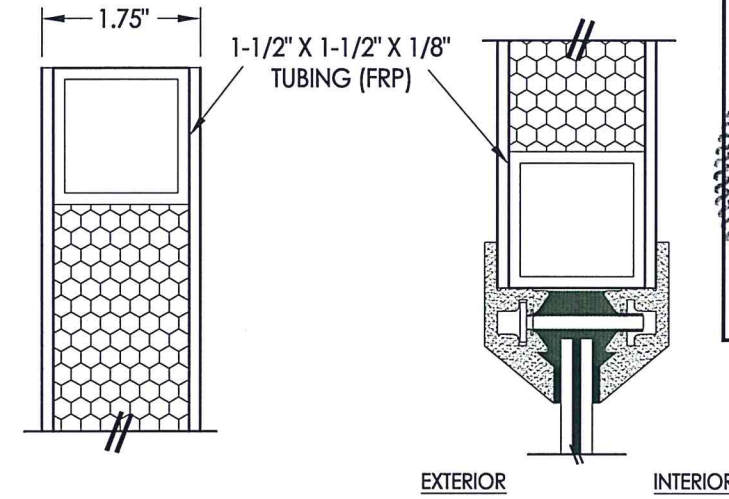
3 2 VERTICAL CROSS SECTION
