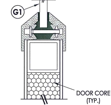
5 2 VERTICAL CROSS SECTION
