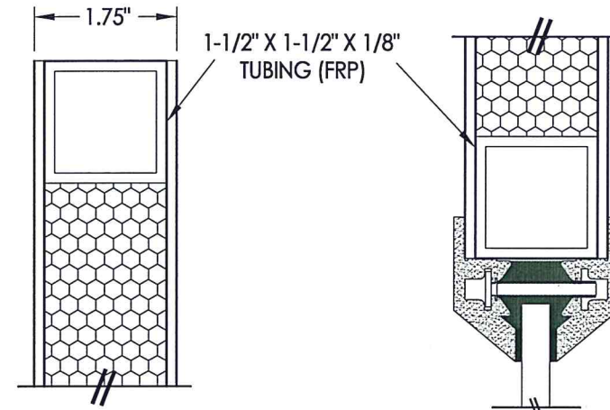
3 2 VERTICAL CROSS SECTION
