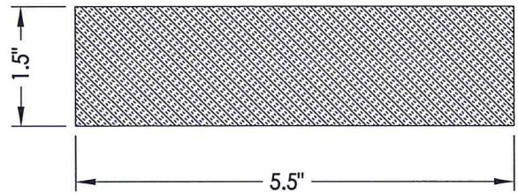
36 REMOVABLE MULLION FRAME BLOCK (FRP) 1.5" WIDE
