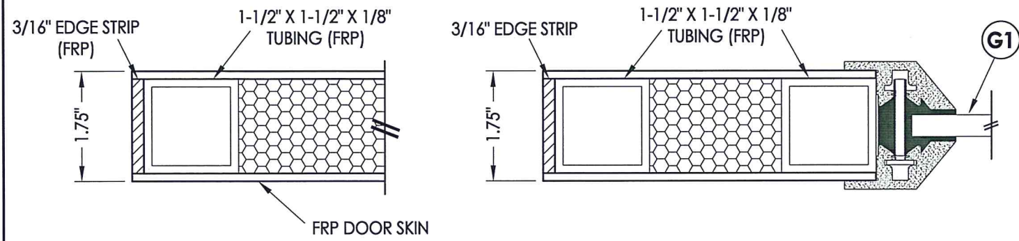
1 2 HORIZONTAL CROSS SECTION
