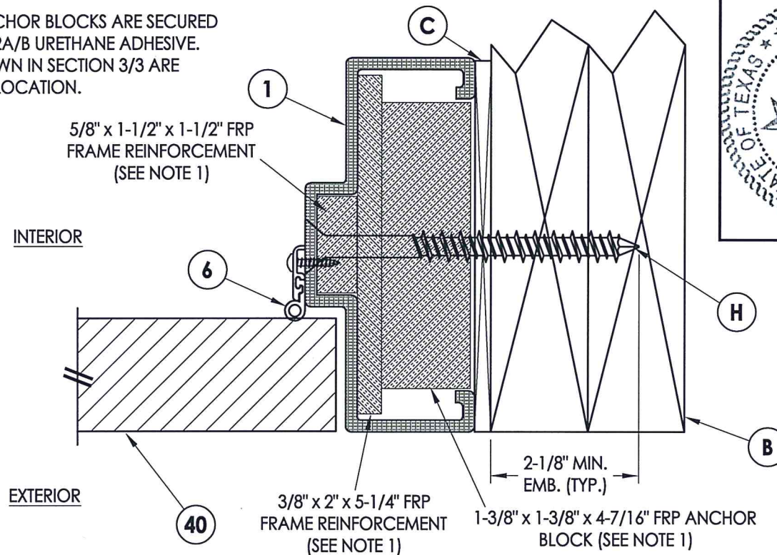
3 HORIZONTAL CROSS SECTION 3 Outswing configuration
