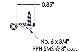
6 WEATHERSTRIP NGP 137N
