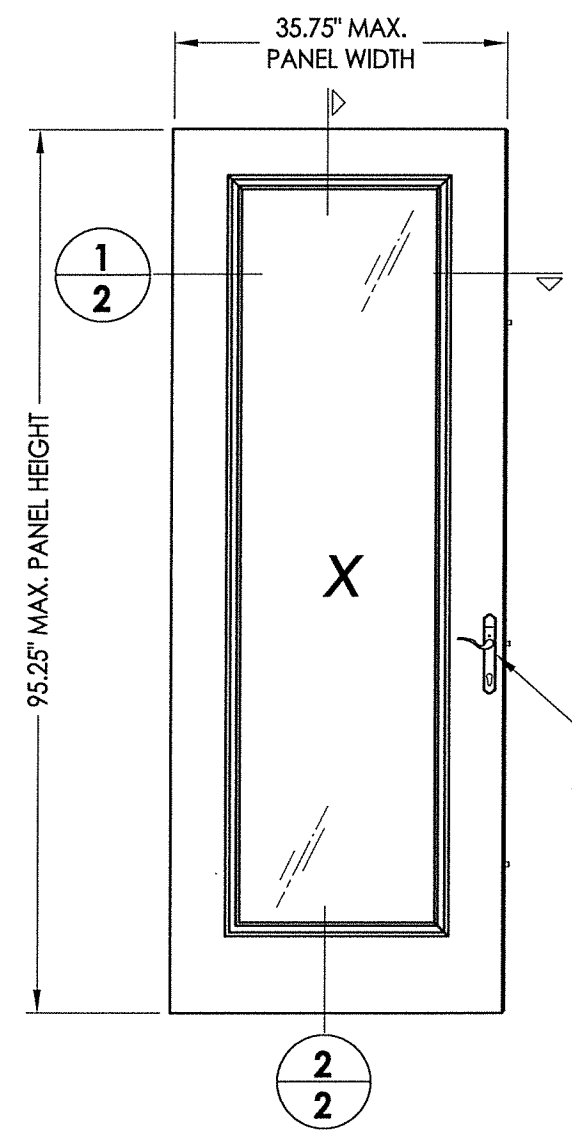
2 2 DOOR PANEL Masonite Steel (Wood Edge)
