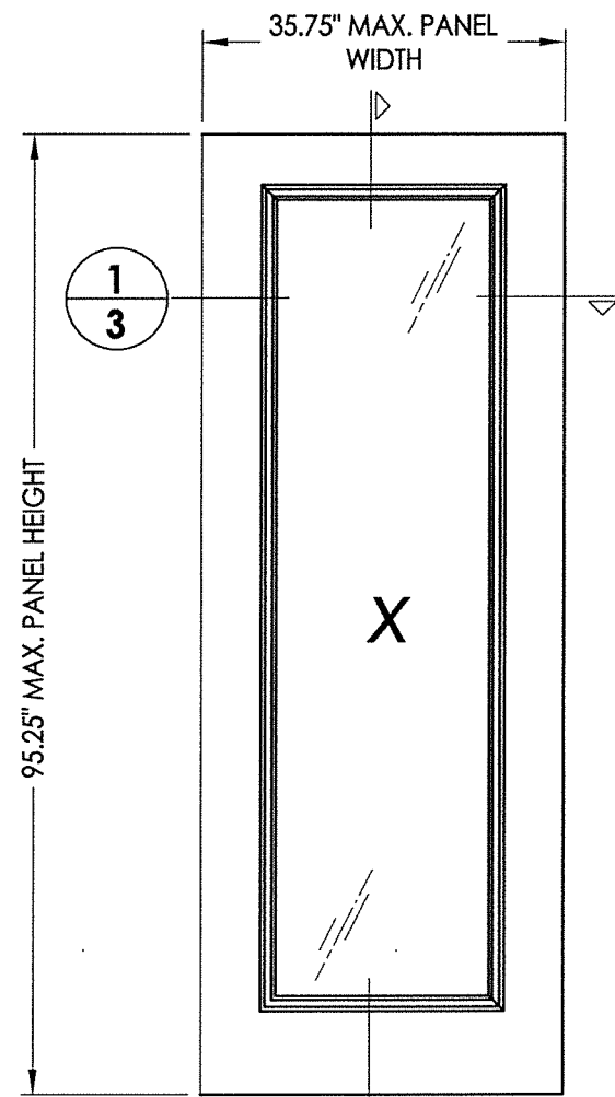
2 3 SIDELITE PANEL Masonite Steel (Wood Edge)
