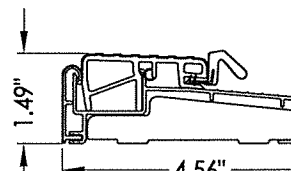
11 OUTSWING THRESHOLD ZOB4565
