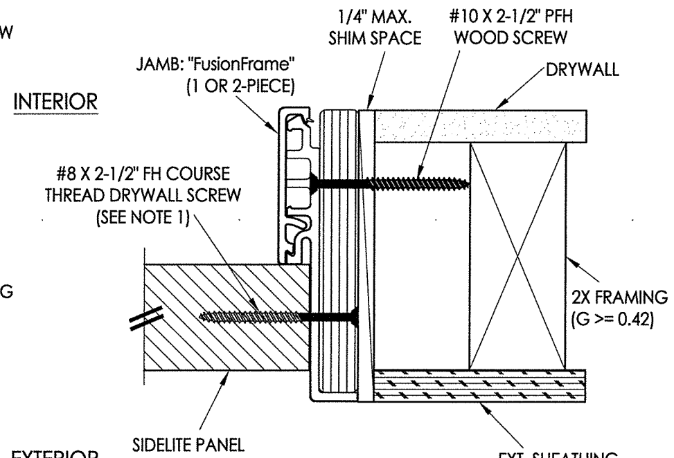
5 HORIZONTAL CROSS SECTION 5 Outswing shown - Inswing also approved
