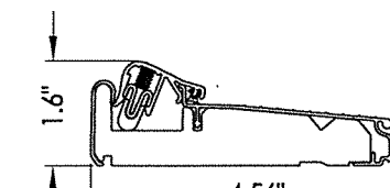
9 INSWING ARTICULATING THRESHOLD ZAC4565FN
