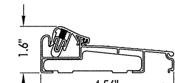
8 INSWING ARTICULATING THRESHOLD ZAC4565
