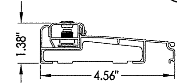
3 INSWING ADJUSTABLE THRESHOLD ZAI4565
