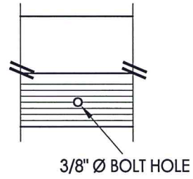
ASTRAGAL BOLT DETAIL Strike Plate @ Head
