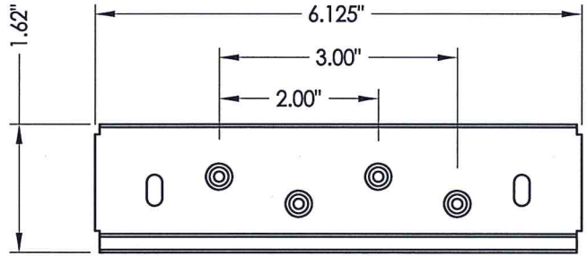
3 HINGE REINFORCEMENT
