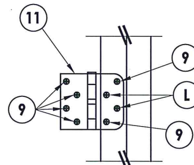
HINGE DETAIL
