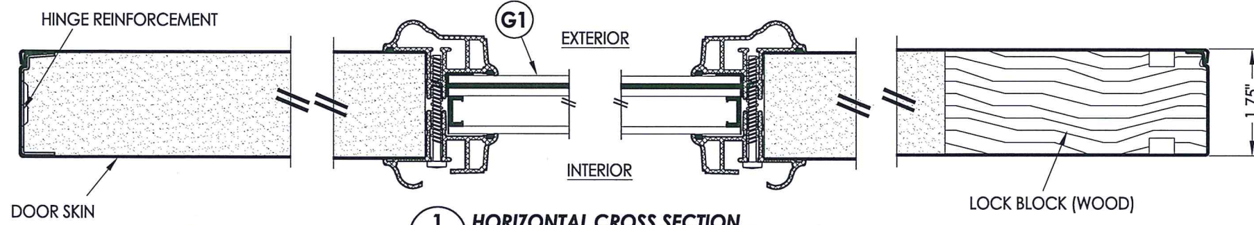
1 2 HORIZONTAL CROSS SECTION
