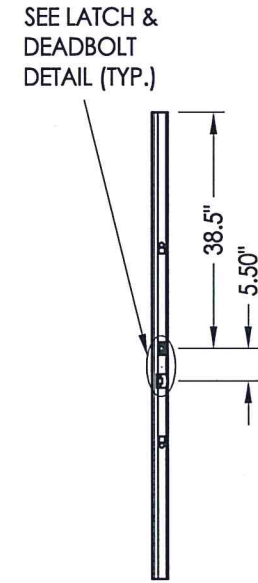
ASTRAGAL STRIKE
