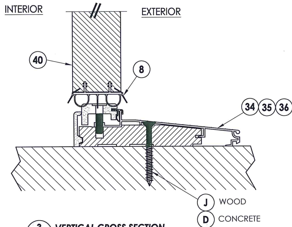
3 6 VERTICAL CROSS SECTION Inswing configuration
