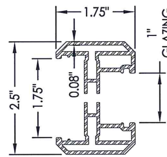
ODL LITE FLAT FRAME 1" GLAZING
