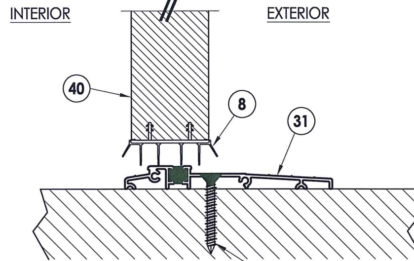
4 6 VERTICAL CROSS SECTION Inswing configuration
