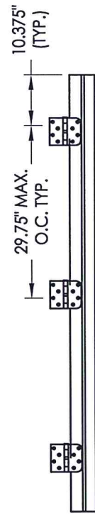
HINGE LOCATIONS
