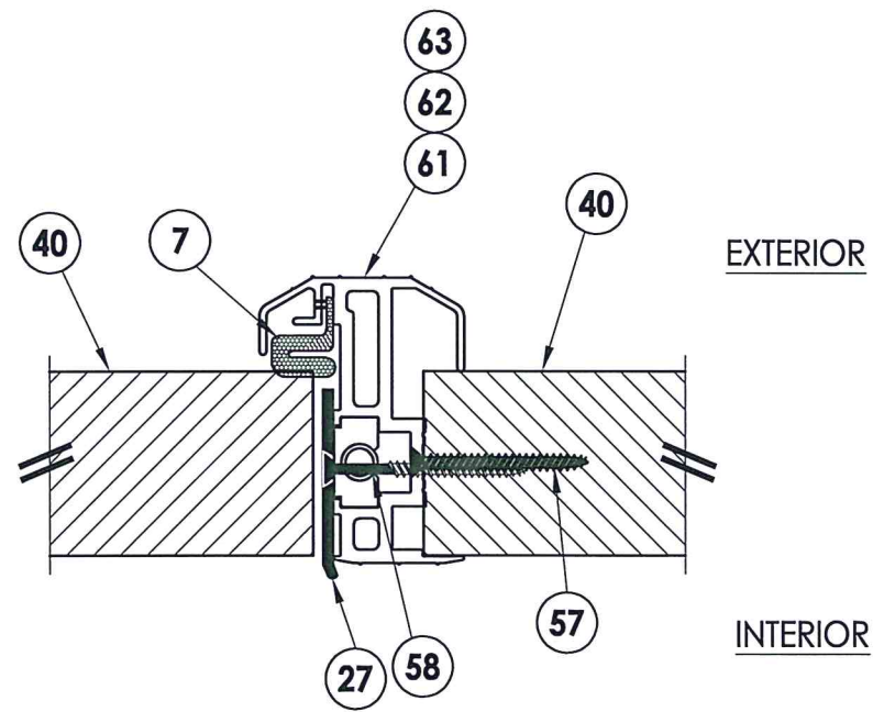
3 HORIZONTAL CROSS SECTION 5
