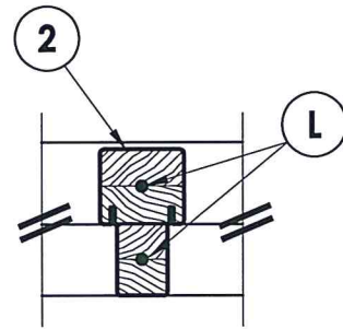
INTEGRAL MULLION ATTACHMENT DETAIL
