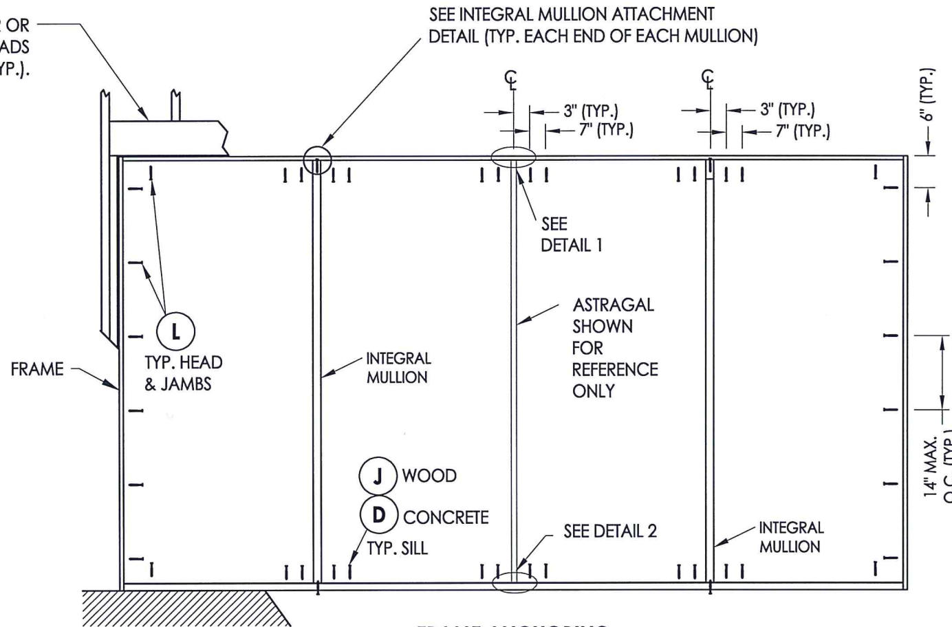
FRAME ANCHORING OXO
