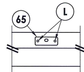
DETAIL 1 Astragal strike @ head
