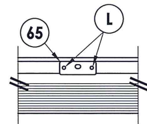
DETAIL 2 Astragal strike @ sill (inswing)
