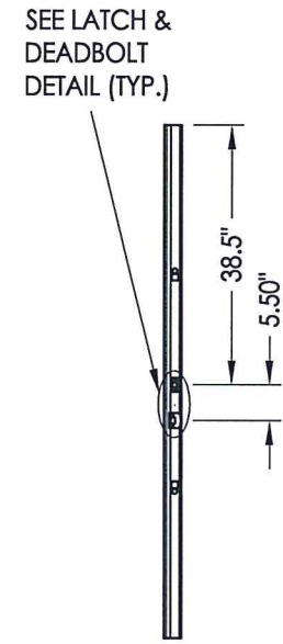
ASTRAGAL STRIKE
