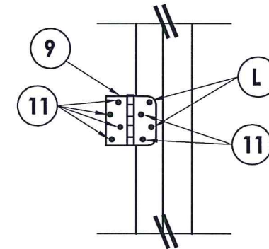
HINGE DETAIL
