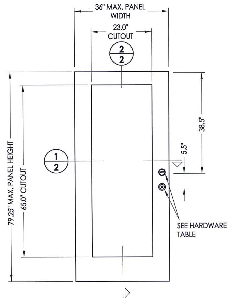
40 DOOR PANEL Fiber Classic (Therma-Tru)
