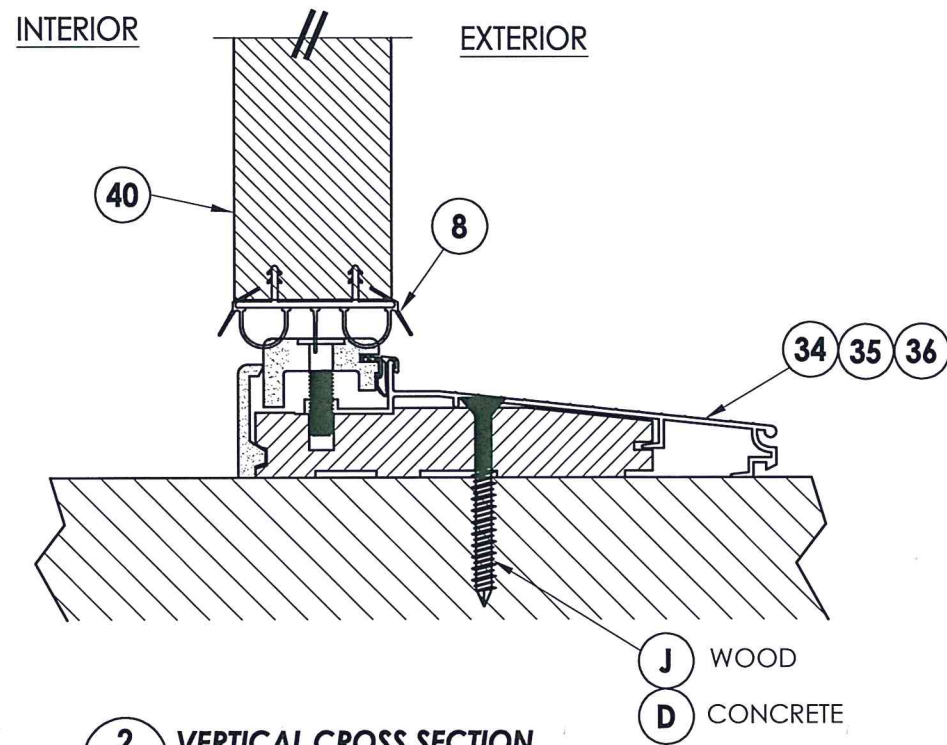
2 6 VERTICAL CROSS SECTION Inswing configuration
