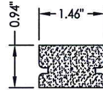
46 DOOR TOP RAIL (CLASSIC CRAFT & RUSTIC)
