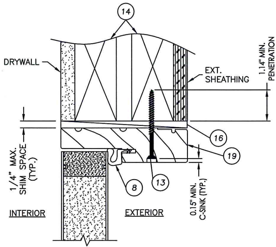
1 VERTICAL CROSS SECTION 6 INSWING SHOWN (OUTSWING ALSO APPROVED) ("SMOOTH STAR SERIES" SHOWN)
