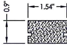
2 DOOR TOP RAIL (SMOOTH STAR)
