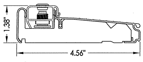
4 INSWING ADJUSTABLE THRESHOLD ZAIAA4565FN MAX. DESIGN PRESSURE = +40/-45 PSF
