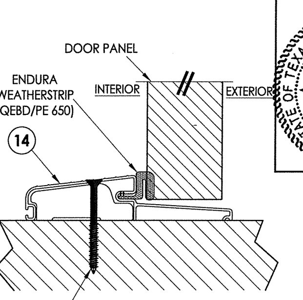
#10 X 2.5" PFH WOOD SCREW OR 1/4" X 2-3/4" ELCO OR ITW CONCRETE SCREW 4 VERTICAL CROSS SECTION 7 Inswing Adjustable Threshold
