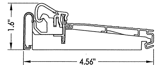
10 INSWING ARTICULATING THRESHOLD ZAC4565RDS MAX. DESIGN PRESSURE = +40/-45 PSF
