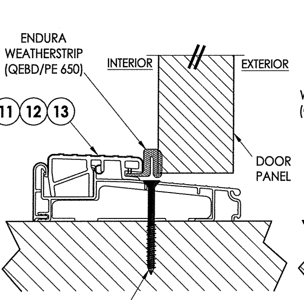
#10 X 2.5" PFH WOOD SCREW OR 1/4" X 2-3/4" ELCO OR ITW CONCRETE SCREW 3 VERTICAL CROSS SECTION 7 Inswing Adjustable Threshold
