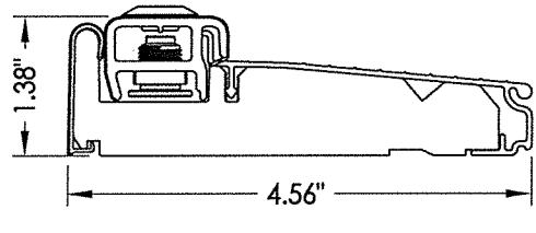
2 INSWING ADJUSTABLE THRESHOLD ZAI4565FN MAX. DESIGN PRESSURE = +40/-45 PSF
