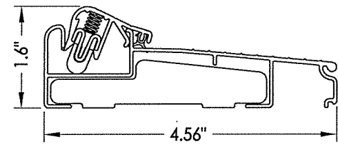
8 INSWING ARTICULATING THRESHOLD ZACLA4565 MAX. DESIGN PRESSURE = +40/-45 PSF
