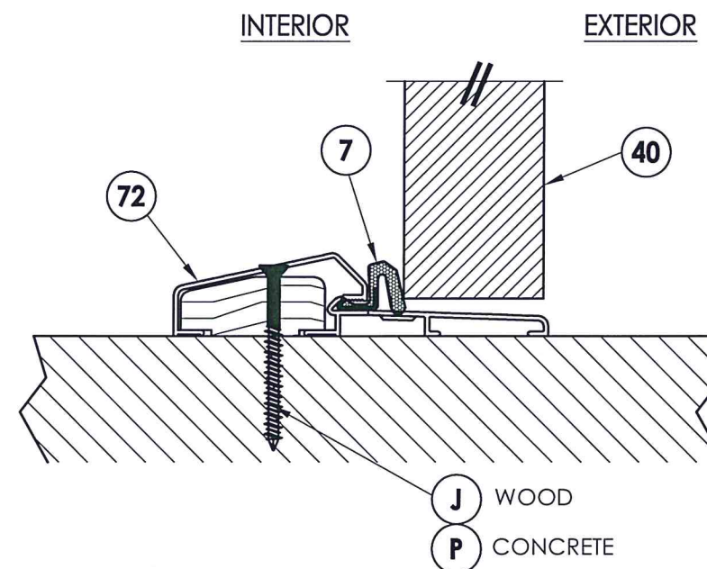
4 VERTICAL CROSS SECTION 6 Outswing configuration
