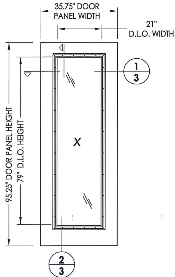
50 SIDELITE PANEL
