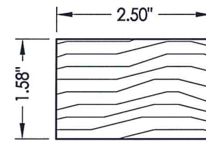
3C STILE Wood Reinforcement (S.G. >= 0.42)
