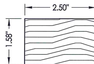
2C LATCH & HINGE STILE Wood Reinforcement (S.G. \geq 0.42 )
